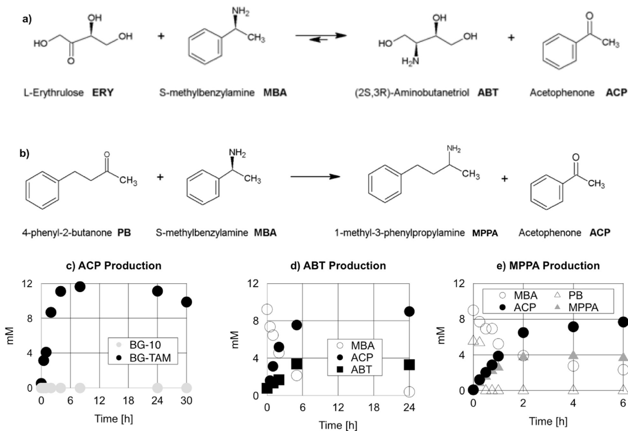
Fig. 2. Transaminase activity in BG-TAM whole cells cultivated in shake flasks. Reaction schemes detail the synthesis of ABT (a) and MPPA (b). Level of ACP generated by strains BG-10 and BG-TAM fed 10 mM MBA and 30 mM ERY as substrates (c). Production of ABT by strain BG-TAM fed 10 mM MBA and 30 mM ERY (d). Production of MPPA by strain BG-TAM fed 10 mM MBA and 10 mM PB (e). Cell concentration normalised to OD_{600} = 39 in all assays. The symbol keys for the graphs obstruct no data points.
