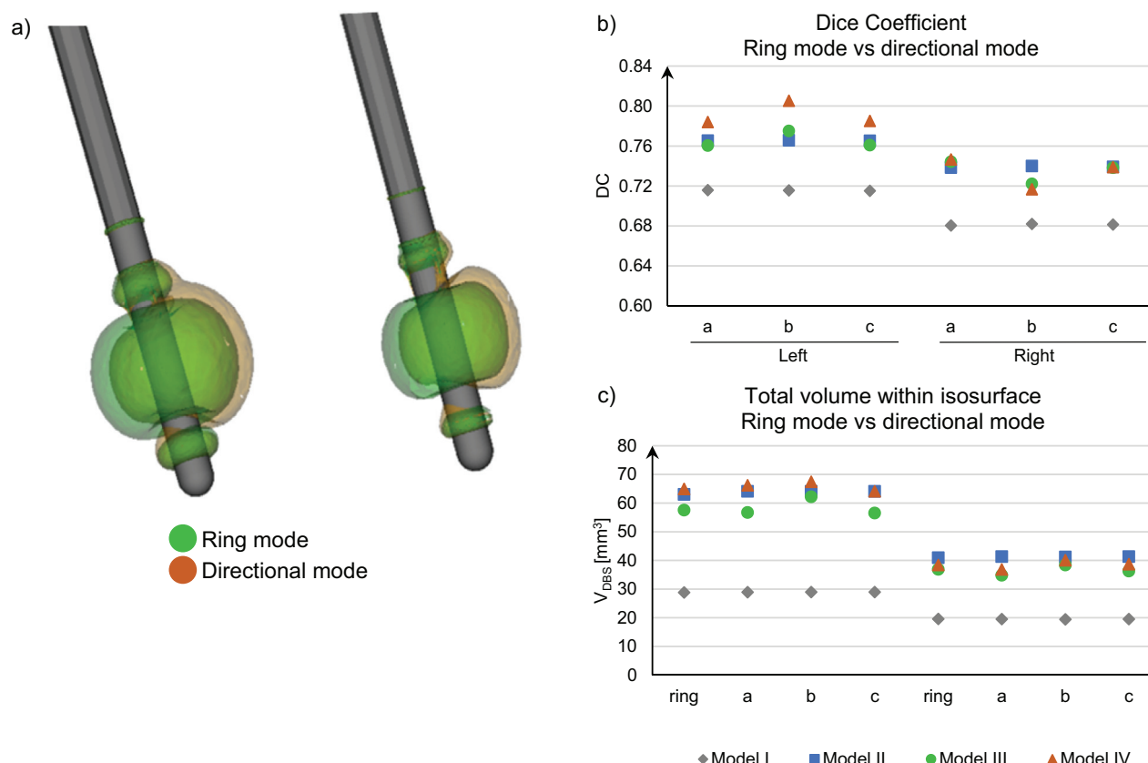
Fig. 10. V_{DBS} comparing ring mode and directional mode in Patient 4, (a) Visualization of the isosurface (0.2 V/mm) in ring mode (green) and using directional mode (segment a, orange) from simulation with Model III, (b) DC comparing ring mode and each segment and (c) plots the total volume of the V_{DBS} . (For interpretation of the references to colour in this figure legend, the reader is referred to the web version of this article.)
