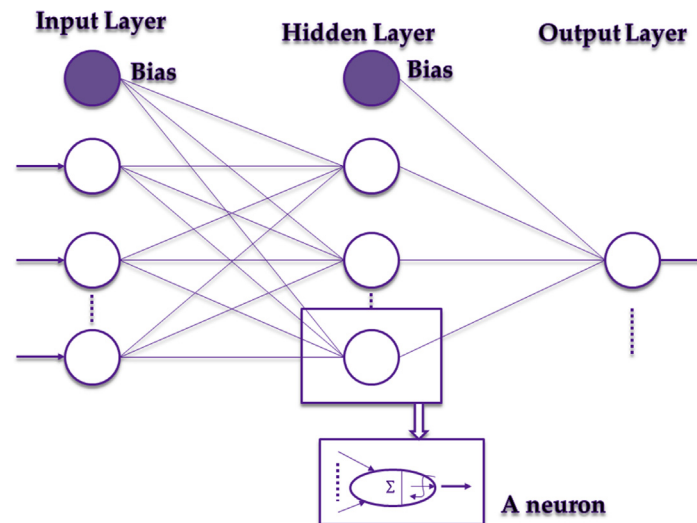
Fig. 4. Typical structure of a multilayer feed-forward ANN [Adapted from Oyeboode (2014)].
