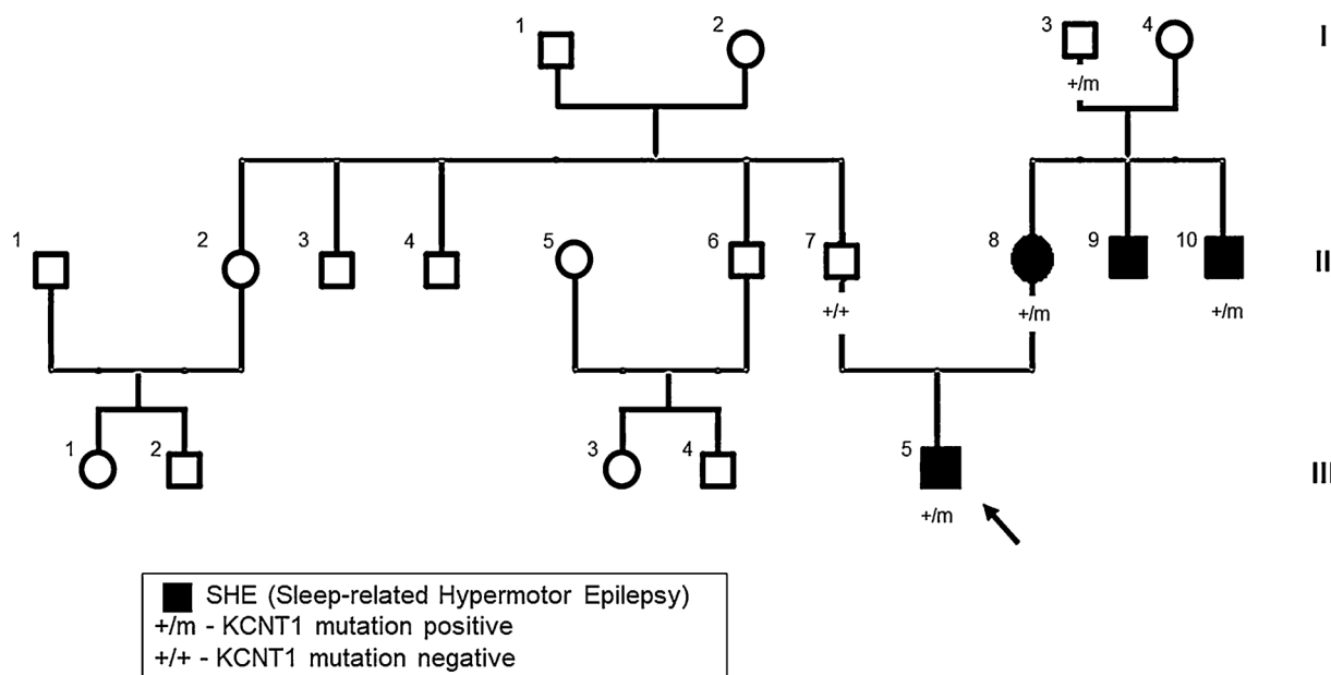
Fig. 1. Family Pedigree.
