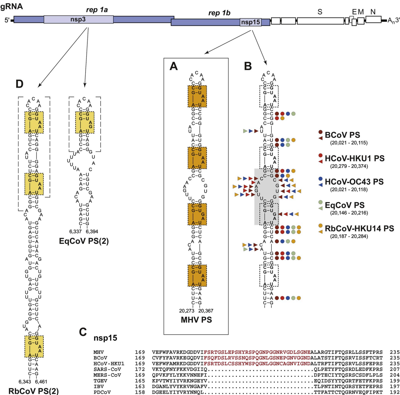
Fig. 2. Betacoronavirus lineage A packaging signals. Top , a map of the lineage A betacoronavirus genome, showing the loci of PS and PS-like elements. (A) Structure of the MHV PS, modeled by Chen et al. (2007) . Repeat units are highlighted in orange. (B) Phylogenetic conservation of the PS among lineage A betacoronaviruses. Circles denote basepairs in double-stranded sections that co-vary between MHV and one of the other viruses; additional base-pairing covariation is found among different strains of MHV and of HCoV-HKU1 (not shown). Triangles denote bases in single-stranded sections that differ from MHV; the shaded rectangle indicates the part of the structure that is deleted in ECoV. (C) Amino-acid alignment of part of the nsp15 subunit of the replicase-transcriptase. Highlighted in red is the segment encoded by the PS of lineage A betacoronaviruses. This segment is absent from all other lineages and genera, here represented by SARS-CoV (betacoronavirus, lineage B), MERS-CoV (betacoronavirus, lineage C), TGEV (alphacoronavirus), IBV (gammacoronavirus), and PdCoV (deltacoronavirus). (D) Upstream PS-like structures, denoted PS(2), in RbCoV and ECoV. In each, broken-line brackets show the region that is a duplication of PS sequence in nsp15; repeat units are highlighted in yellow. GenBank accession numbers for the sequences shown: MHV, AY700211; BCoV, U00735; HCoV-HKU1, AY597011; HCoV-OC43, AY903460; ECoV, EF446615; RbCoV-HKU14, JN874559; SARS-CoV, AY278741; MERS-CoV, JX869059; TGEV, AJ271965; IBV, AJ311317; PdCoV, JQ065042.
