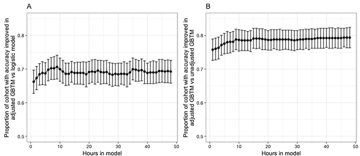
Fig. 4 – Proportion of subjects each hour for whom accuracy of predicted outcome was improved in the adjusted GBTM compared to the logistic model (A) or unadjusted GBTM (B). Confidence bars show the exact binomial 95% confidence interval around the proportion point estimate.
