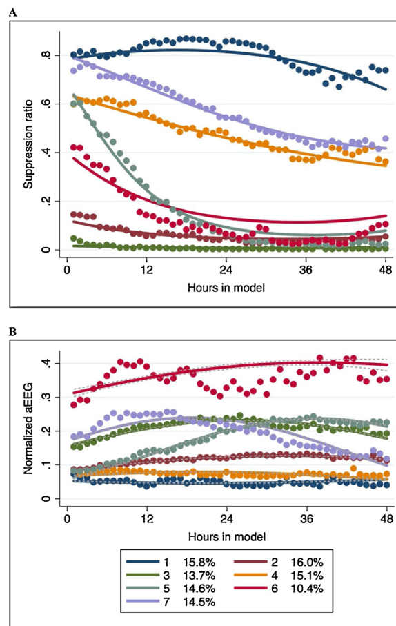
Fig. 2 – Final seven group multi-trajectory model of normalized suppression ratio (A) and aEEG (B) over time.
