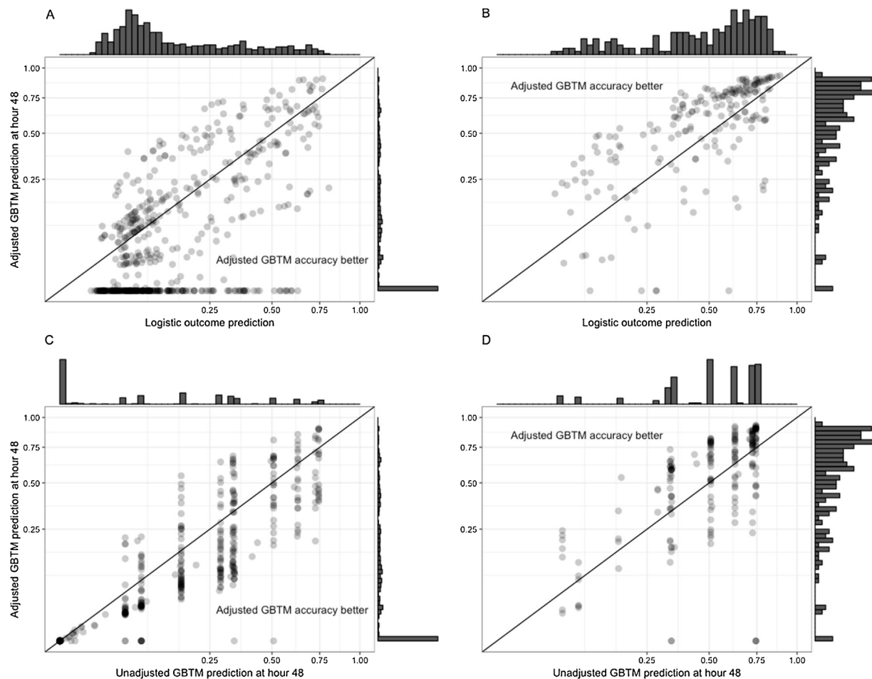
Fig. 3 – Patient-specific differences between outcome models at hour 48. Prediction from the adjusted GBTM was improved among subjects with unfavorable outcomes when it was lower than that of the logistic (A) or unadjusted GBTM (C) estimates, points falling below the reference line in these panels. By contrast, prediction from the adjusted GBTM was improved among subjects with favorable outcomes when it was higher than the logistic (B) or unadjusted GBTM (D), points falling above the reference line. All axes are shown in a square root scale.
