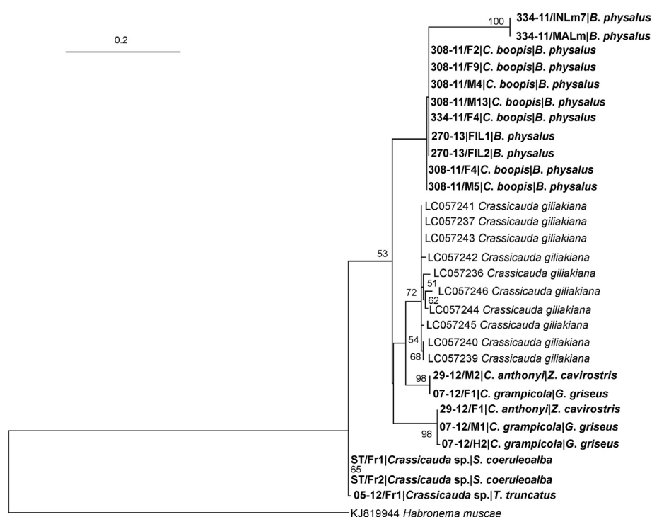
Fig. 5. Maximum likelihood tree (Log-likelihood: -1359.826) obtained from cox1 alignment. The tree was arbitrarily rooted on midpoint. Bootstrap support values ( \geq 50\% ) are provided near the corresponding node. The scale bar represents 0.2 substitutions/site. Newly determined sequences are in bold.
