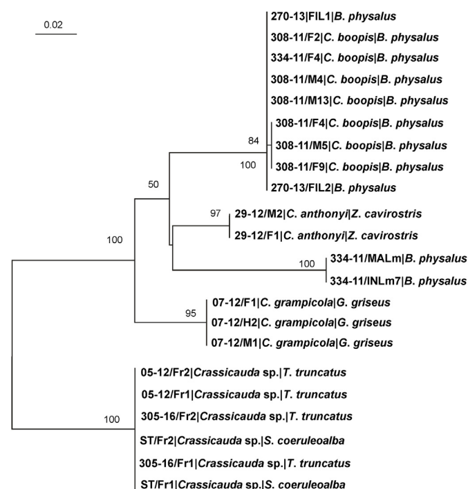
Fig. 4. Maximum likelihood tree (Log-likelihood: -1044.368) obtained from ITS2 alignment. The tree was rooted on midpoint. Bootstrap support values ( \geq 50\% ) are provided near the corresponding node. The scale bar represents 0.02 substitutions/site. Newly determined sequences are in bold.
