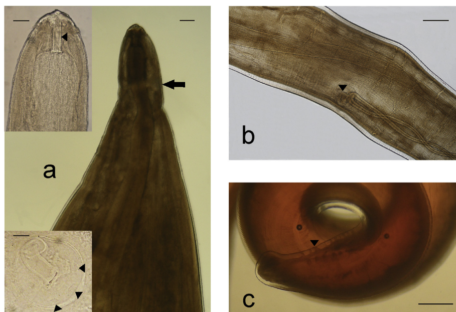
Fig. 1. Adult Crassicauda boopis . a) Female. Cephalic end (bar = 120 \mu m) with particular of the buccal cavity (arrowhead in the upper inset, lateral view; bar = 60 \mu m) and of lateral and submedial cephalic papillae situated along the margin of a cuticular plate (arrowheads in lower inset, apical view; bar = 25 \mu m). b) Female. Paired uteri opening in the vulva (arrowhead) (bar = 600 \mu m). c) Male. Coiled caudal extremity with caudal papillae (arrowhead) (stereomicroscope) (bar = 1 mm).
