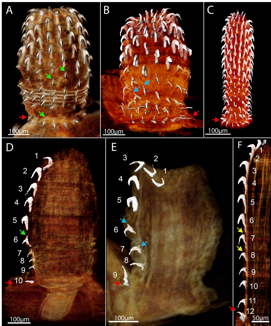
Fig. 2. Proboscis and longitudinal row of hook roots of the three determined Pomphorhynchus species. All images are volume rendering of the 3-D stacks. In volume rendering each grayscale value is assigned a color according to an arbitrary colormap. The depiction depends on which values and how transparent they are displayed. In the present images a glow color map is used, which assigns graded colors from black (background) to shades of red-orange-yellow. A. Volume rendering of a confocal laser scan image stack of the proboscis of P. tereticollis . B. Volume rendering of the sectioned proboscis of P. bosniacus including reconstructed hooks as surface rendering. C. Volume rendering of the sectioned proboscis of P. laevis including reconstructed hooks as surface rendering. D–F. Internal view of the sectioned probosces including a single longitudinal row of hooks. D. P. tereticollis . E. P. bosniacus . F. P. laevis . Legend: Red arrow = last circle of hooks; green arrow = extensions on basal hook roots of P. tereticollis ; blue arrow = basal hooks attached in the middle of hook roots of P. bosniacus ; yellow arrow: lack of extensions on basal hook roots of P. laevis . (For interpretation of the references to color in this figure legend, the reader is referred to the Web version of this article.)
