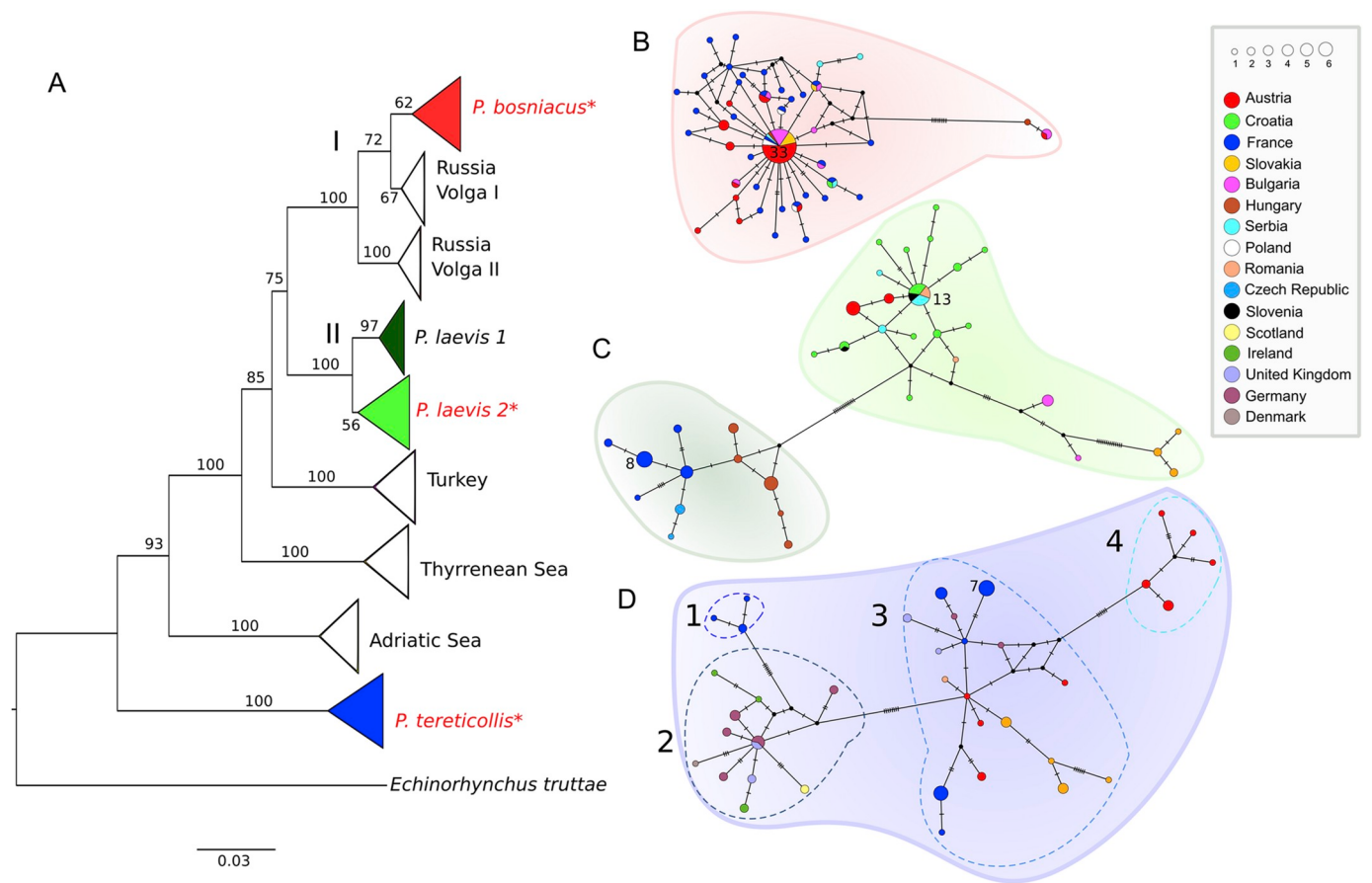
Fig. 3. Phylogenetic relationships between species of the genus Pomphorhynchus based on a 550 bp COI dataset. A. NJ tree showing uncorrected p -distances between species of the genus Pomphorhynchus . Bootstrap values (1000 replicates, in %) are shown next to the nodes. Clade names containing specimens examined in this study are colored in red and marked with an asterisk. The dataset includes sequences generated in this study and sequences obtained from NCBI GenBank. B. Median-joining network of P. bosniacus . One frequent haplotype can be observed (n = 33). Most haplotypes are constituted of 1 sample (see legend), separated by one to two mutation steps from the main haplogroup. Only two haplotypes including sequences from NCBI GenBank are separated by eight mutation steps from the main haplogroup. C. Median-joining network of P. laevis . Two different clades can be distinguished: a Western clade (dark green) and an Eastern clade (light green). Specimens of this study are represented in two separate haplotypes. D. Median-joining network of P. tereticollis . Four different haplogroups can be distinguished, indicated with dotted lines: 1. Specimens from France (Rhône) (NCBI GenBank), 2. Specimens from Northern Europe (NCBI GenBank), 3. Specimens from the Rhine and Carpathians (NCBI GenBank), including specimens of this study, 4. Specimens of this study. Mutation steps are indicated with vertical lines. Black dots represent haplotypes missing in the study sampling. (For interpretation of the references to color in this figure legend, the reader is referred to the Web version of this article.)
