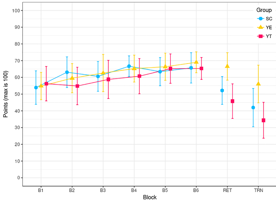
Fig. 2. Mean points (with 95% confidence intervals) scored during the acquisition (B1-B6), retention (RET), and transfer (TRN) phases of the experiment for the self-controlled (SC, blue circles), the traditional yoked (YT, red squares), and the yoked with estimation (YE, yellow triangles) groups. Please refer to online version for references to color. (For interpretation of the references to color in this figure legend, the reader is referred to the web version of this article.)
