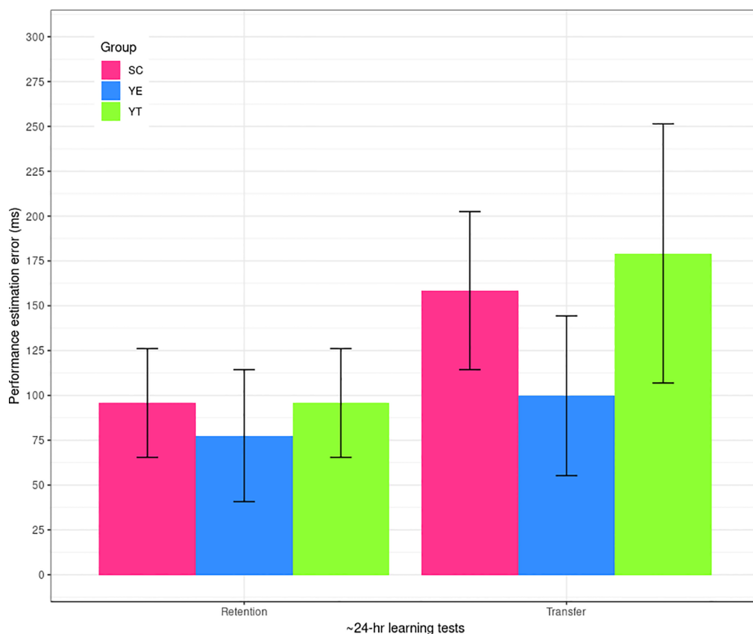
Fig. 7. Mean (with 95% confidence intervals) absolute constant error of performance estimation scores for the SC group (left, red bars), the YE group (middle, blue bars), and the YT group (right, green bars) for the retention and transfer phases of Experiment 2. (For interpretation of the references to color in this figure legend, the reader is referred to the web version of this article.)
