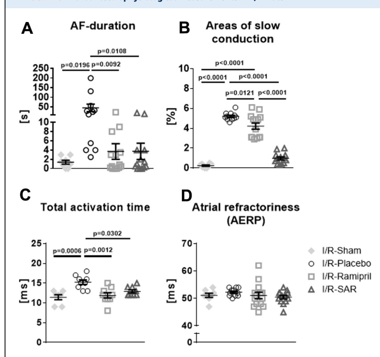
FIGURE 3 Atrial Electrophysiological Measurements in I/R-Rats
