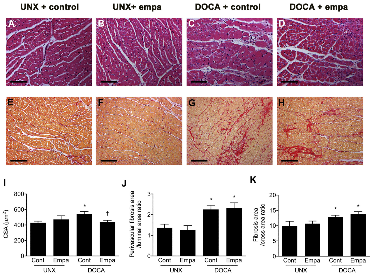
FIGURE 4 Stained Sections
