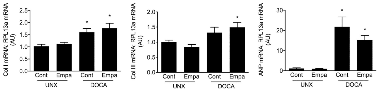
FIGURE 5 Heart Collagen 1 and III, ANP mRNA Levels
