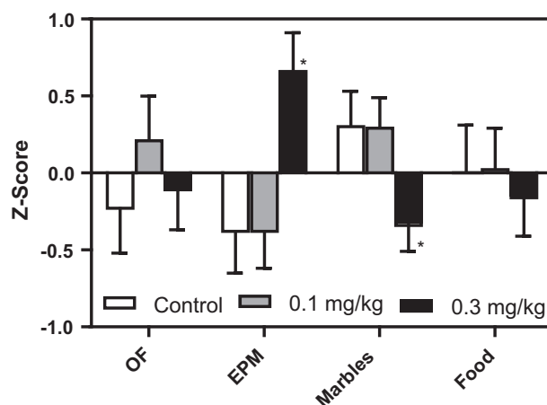
Fig. 1. Effects of asenapine in a battery of tests for anxiety-like behavior. Data presented as mean \pm SEM of Z-scores. * represents statistically significant difference from control based on MANOVA and post-hoc analysis of the raw data. OF = Spontaneous activity in open field; EPM = open/closed arms time ratio in the elevated plus-maze; Marbles = number of marbles covered in the defensive marble burying test; Food = latency to eat in the novelty-induced hypophagia test.
