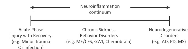
Fig. 1. Neuroinflammation continuum. Neuroinflammation occurs in a continuum. It can result from acute phase injury where recovery to baseline occurs quickly after minor traumatic injury or infections, but when neuroinflammation is sustained, it has widely been associated with neurodegenerative diseases such as Alzheimer’s disease (AD), Parkinson’s disease (PD) and multiple sclerosis (MS). In the middle of this neuroinflammation continuum are chronic sickness behavior disorders with no apparent underlying neurodegeneration (ME/CFS, GWI and chemobrain represent examples of distinct diseases in this non-neurodegenerative category).
