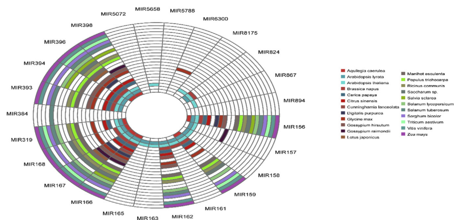
Fig. 2. Circular heat map of conserved miRNAs identified in ginseng among different model plants. Each color represents a plant species and white color represents the absence of miRNA. MiRNA that was found in at least 9 plants was considered as conserved.
