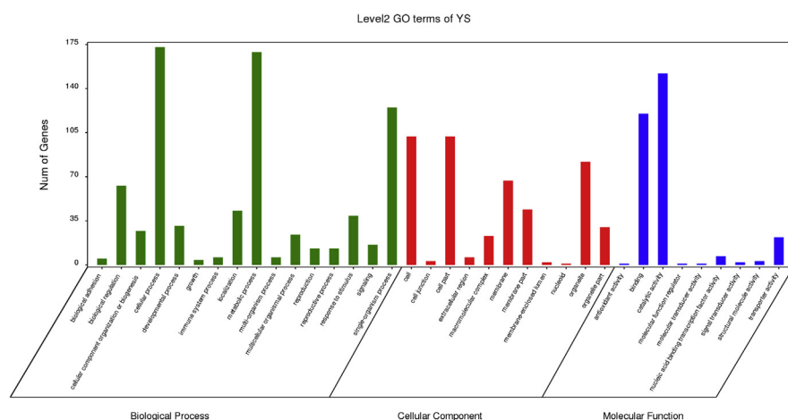
Fig. 3. GO enrichment analysis of all predicted target genes in ginseng.
