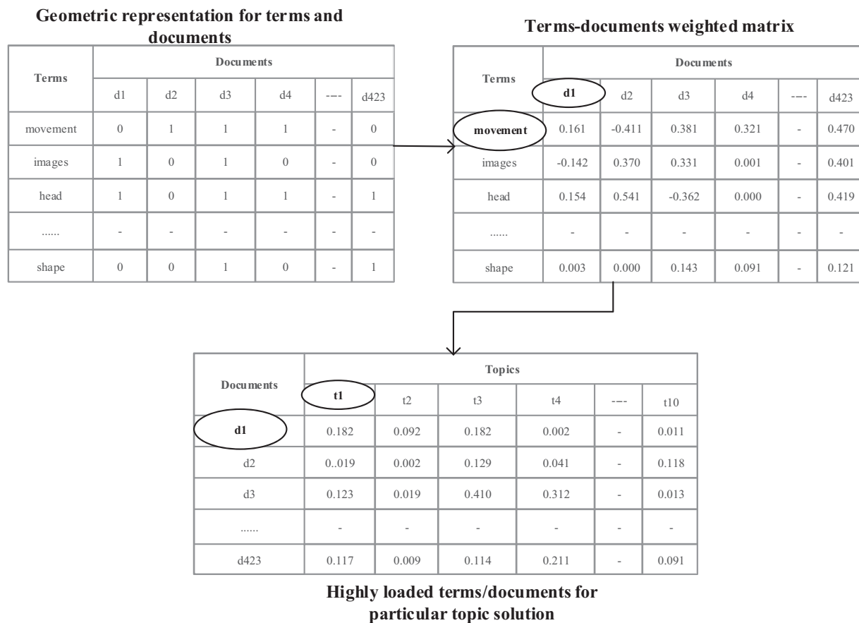
Figure 2. Two dimensional representation and documents (columns) for a particular topic solution.
