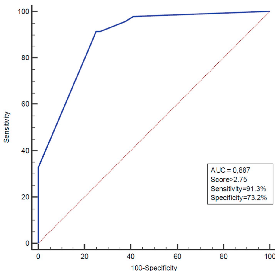
Fig. 1. ROC analysis identify the score with the highest sensitivity and specificity. A score > 2.75 predicted evolution to SSc in patients with UCTD-risk-SSc with 91.3% sensitivity and 73.2% specificity.
