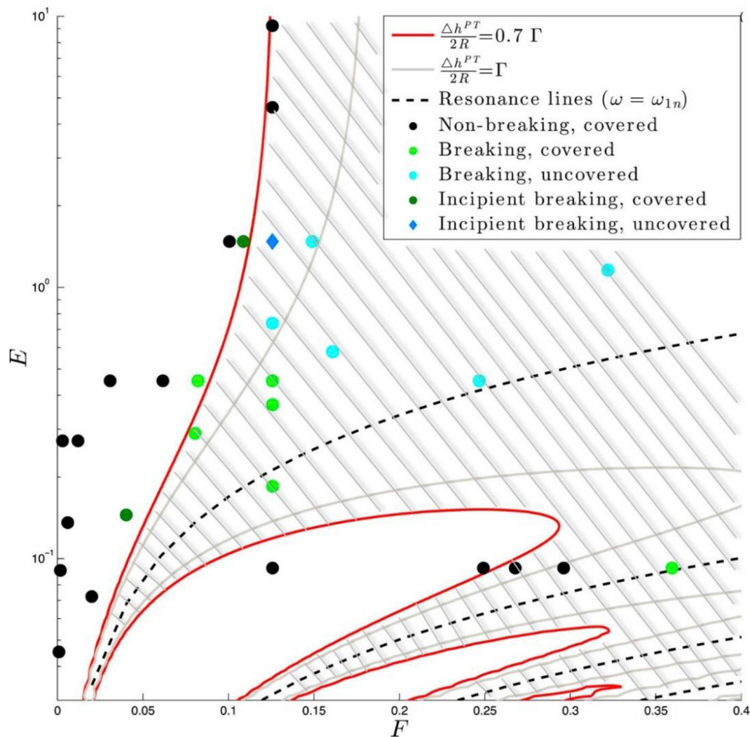
Fig. 2. Classification of the different wave-breaking regimes.
