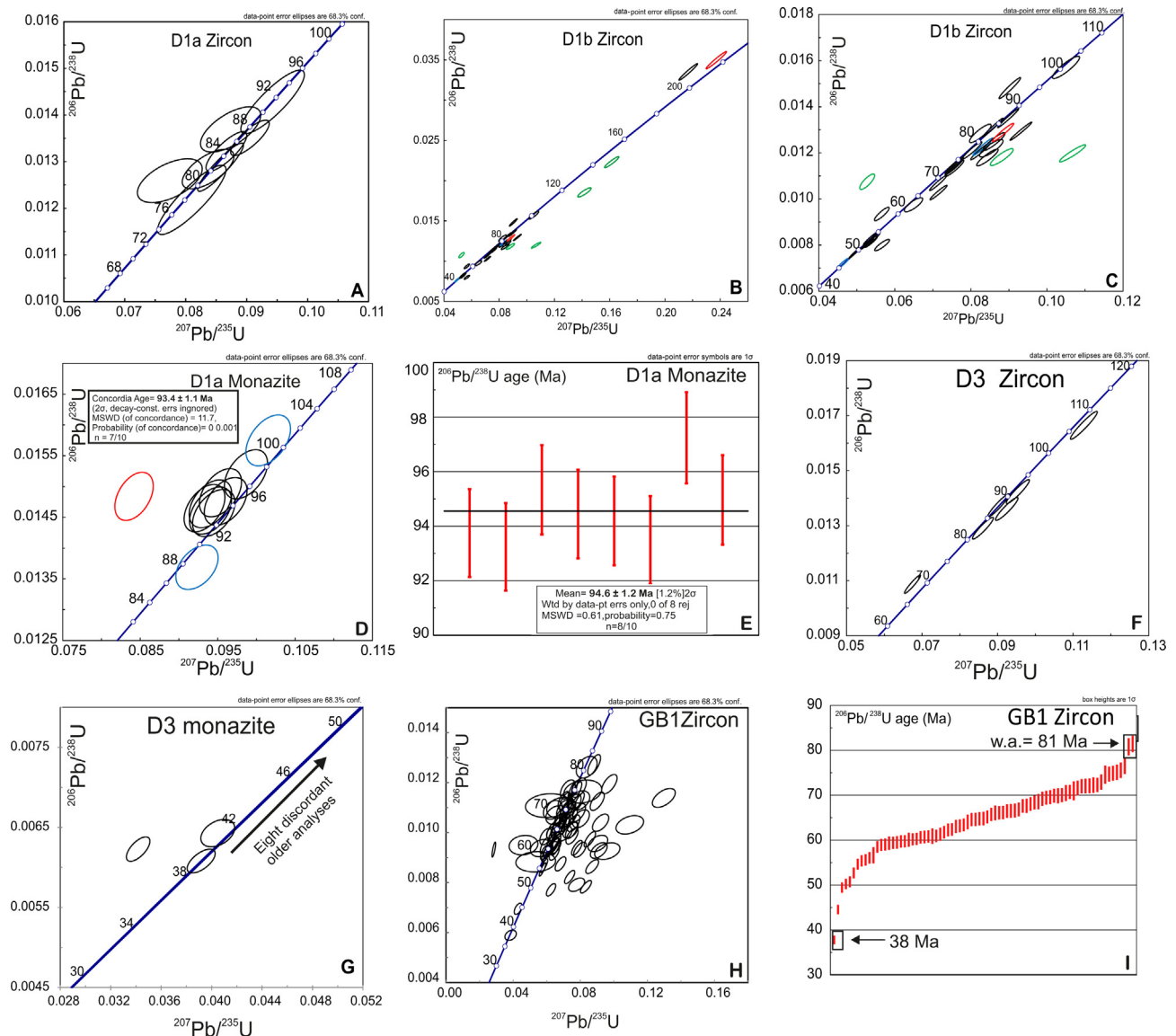
Fig. 6. U–Pb concordia and ^{206}\text{Pb}/^{238}\text{U} weighted average diagrams of zircons and monazites. (A) Age of zircons from felsic sample D1a using a Nu Plasma HR multicollector ICP-MS. (B and C) Age of zircons from felsic sample D1b using a Nu Plasma AttoM single collector ICP-MS. (D) Concordia age of monazites from D1a. Blue and red colours indicate analyses omitted from age calculation. (E) Weighted average ^{206}\text{Pb}/^{238}\text{U} age of monazites from sample D1a. (F) Age of zircons from D3. (G) Age of monazites from D3. (H) Age of zircons from GB1. (I) All the analyses of GB1 indicating the youngest and oldest ages (w. a. = weighted average). The blue, green and red colours in error ellipses refer to analyses which come from the same grain, respectively.
