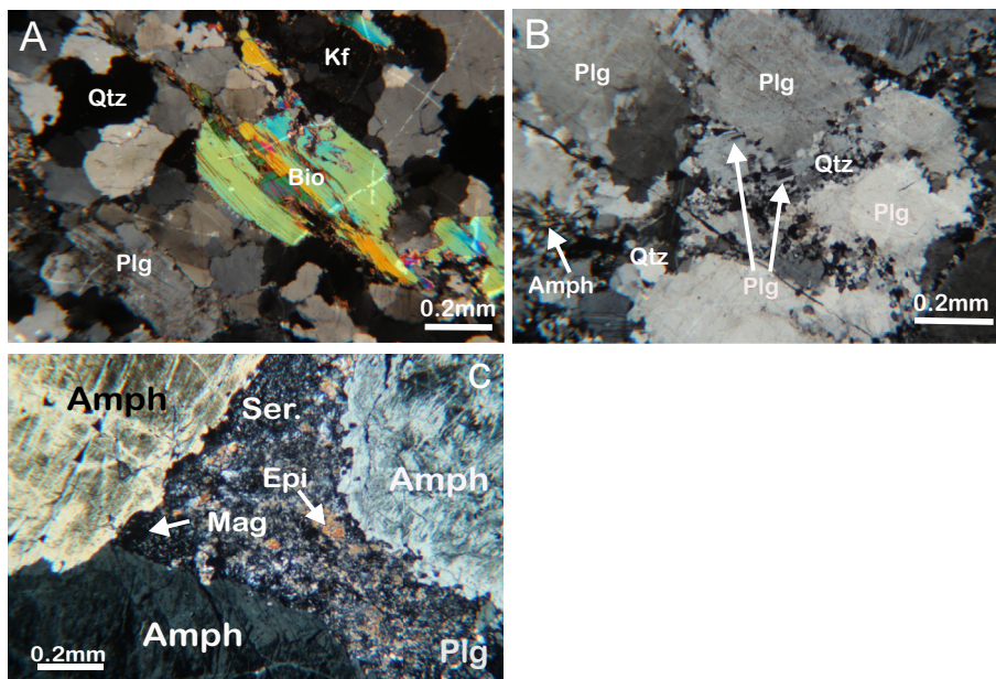
Fig. 4. Photomicrographs from the Mawat ophiolite, cross-polarized light: (A) Felsic dyke D1 with hybi-diomorphic granular texture. (B) Felsic dyke D3 with coarse-grained porphyritic texture of plagioclase and quartz. (C) Coarse-grained amphibole and plagioclase in the pegmatitic gabbro. Plagioclase show weak twin lamellae and partially altered to sericite. Amph = amphibole; Bio = biotite; Epi = epidote; Mag = magnetite; Plg = plagioclase; Qtz = quartz, Kf = k-feldspar, and Ser = sericite.
