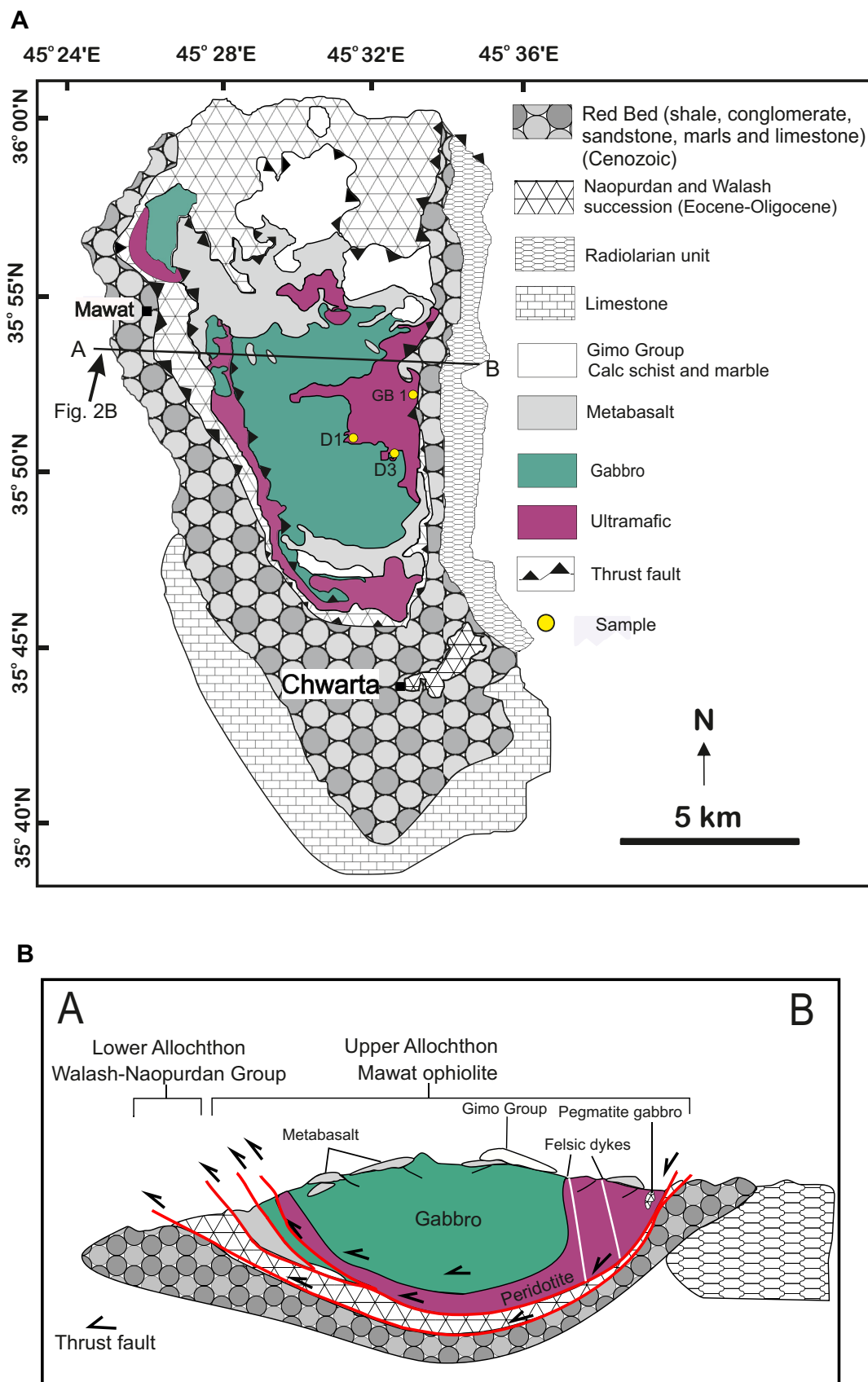
Fig. 2. (A) Simplified geological map of the Mawat ophiolite (modified from Aziz, 2008 ). (B) Simplified cross-section of the Mawat ophiolite along the traverse A-B (modified from Jassim and Goff, 2006 ). For location and legend see Fig. 2A .
