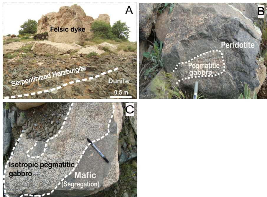
Fig. 3. Field photographs from the Mawat ophiolite, showing (A) Felsic dyke intruding the mantle peridotite (serpenitized harzburgite) and dunite. (B) Pegmatitic gabbro within peridotite. (C) Isotropic pegmatitic gabbro and fine-grained mafic segregation.
