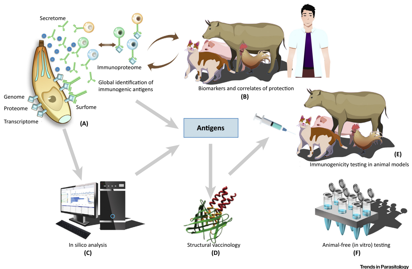
Figure 3. An Integrated Strategy for the Discovery and Testing of Vaccine Candidates in the Postgenomics era. (A) Discovery of novel vaccine Toxoplasma gondii candidates. Vaccine candidates can be identified through analysis of the T. gondii 's genome (the complete genetic content of T. gondii ), transcriptome (the complete set of RNA transcripts expressed by T. gondii under a certain condition), proteome (the complete set of proteins expressed by T. gondii under a certain condition), secretome (the complete set of proteins secreted by T. gondii under a certain condition), and surfome (the subset of proteins that are surface exposed). In parallel, the immunoproteome (the set of antigens that interact with the host immune system) can provide a panoramic view of the spectrum, intensity, and dynamics of antibodies binding to T. gondii proteins, revealing their immunogenicity potential. (B) Toxoplasmosis biomarkers and immune-correlates of protection across vulnerable host species. Further characterization of protective immune response is required in order to identify novel unambiguous markers that correlate with, and predict, vaccine-induced protective immunity against T. gondii infection. (C) Computational ( in silico ) analysis (e.g., comparative genomics, population genetics, stage-specific antigen, and prediction of B and T cell epitopes) can facilitate all aspects of preclinical and clinical vaccine development. (D) The structural vaccinology (the 3D structure of proteins, in particular the structural epitopes of immunogenic antigens) can be a useful aid in any future T. gondii vaccine development. (E) Experimental infection models are crucial for testing the clinical efficacy of T. gondii vaccine. (F) Animal-free ( in vitro ) systems can provide preclinical proof-of-concept in support of vaccine development.
