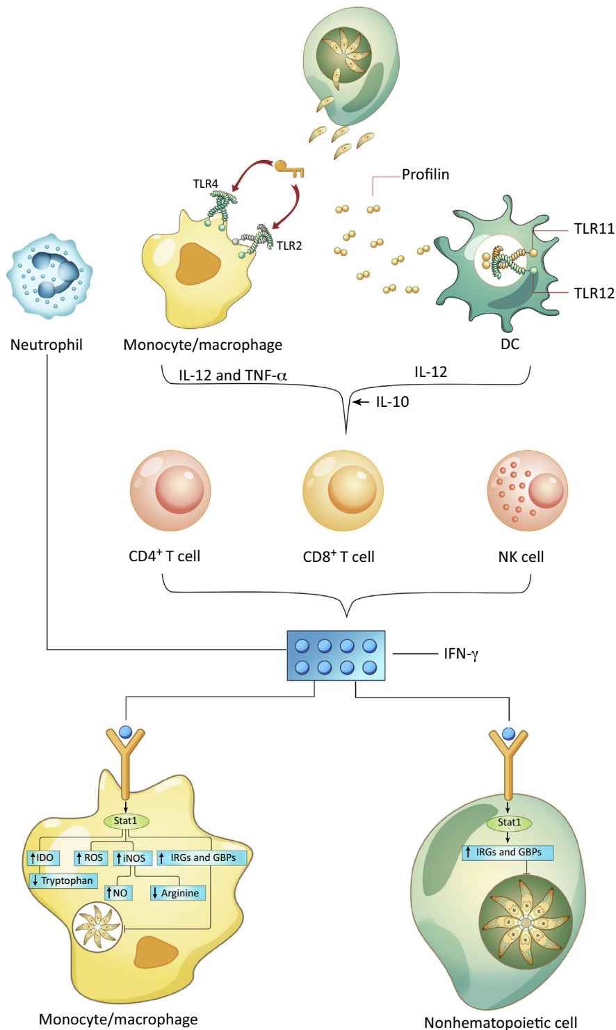
Figure 2. Host Immune Responses against Toxoplasma gondii . Chemokines secreted from cells at the site of infection trigger the recruitment of neutrophils, dendritic cells (DCs), monocytes, and macrophages to the site of infection.
