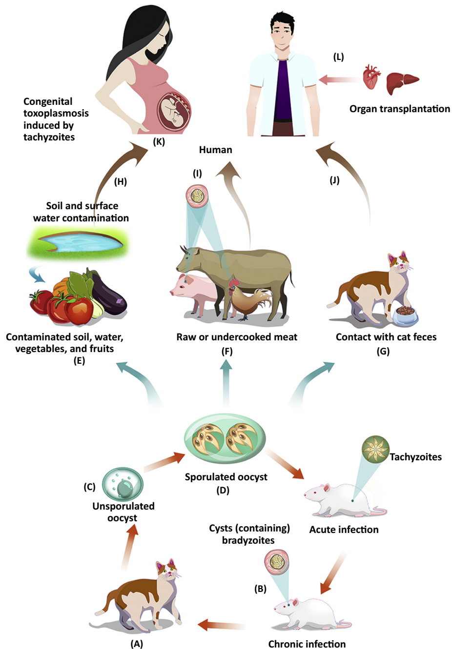
Figure 1. The Two-Host, Predator-Prey, Life Cycle of Toxoplasma gondii . (A) Members of the family Felidae (domestic and wild cats) are the only known definitive hosts of T. gondii . (B) Cats become infected after ingestion of viable tissue cysts. (C) Cats shed unsporulated oocysts in their feces into the environment. (D) After shedding, oocysts mature in the environment into infective (sporulated) oocysts. Oocysts are able to survive in the environment for long periods of time, and the sporulated oocysts can contaminate soil, water, vegetables, and fruits (E), providing a route of infection to a wide range of intermediate hosts (F) and cats (G). T. gondii infection is initiated in humans by ingestion of oocysts in contaminated food or water (H) or ingestion of viable tissue cysts in raw or undercooked meat (I). Other means of infection include contact with cats (J), mother-to-child transmission (K), or by organ transplantation (L). Shortly after (Figure legend continued on the bottom of the next page.)
