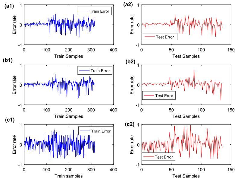
Figure 7. Error rate of both Train and Test data for original PSO operators (PSO) (a1-a2), Mantegna Lévy Flight (MLF) (b1-b2), and Neighborhood Search (NS) (c1-c2).
