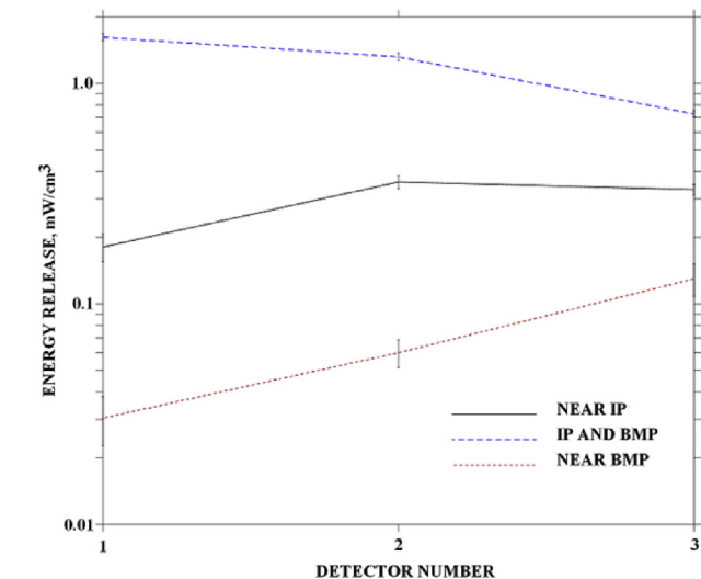
Fig. 8. Neutron and secondary photon energy release in the case on the external contour of TMFC located near the IP, between the IP and the BMP, and near the BMP.
