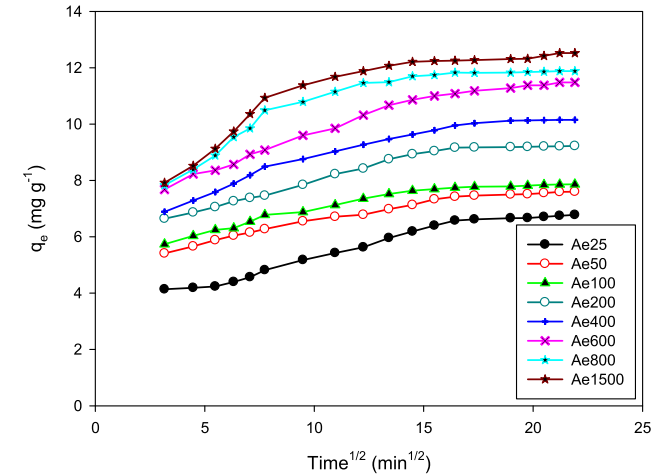
Fig. 12. Experimental data adjusted to the intraparticle model in Ni(II) adsorption on carbon aerogels. C_0 = 500 \text{ mg}\cdot\text{L}^{-1} , T = 25^\circ\text{C} . 1 \text{ g}/500 \text{ mL} . \text{pH} = 5.0 .
