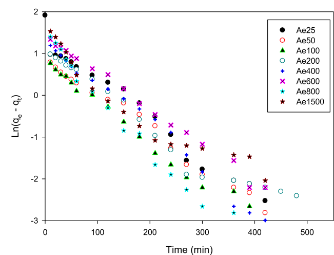
Fig. 10. Experimental data adjusted to the pseudo-first order model - Lagergren in the adsorption of Ni(II) on carbon aerogels. C_0 = 500 \text{ mg}\cdot\text{L}^{-1} , T = 25^\circ\text{C} . 1 \text{ g}/500 \text{ mL} . \text{pH} = 5.0 .
