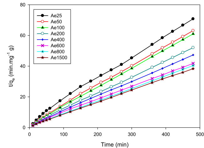
Fig. 11. Experimental data adjusted to the pseudo second order model in Ni(II) adsorption on carbon aerogels. C_0 = 500 \text{ mg}\cdot\text{L}^{-1} , T = 25^\circ\text{C} . 1 \text{ g}/500 \text{ mL} . \text{pH} = 5.0 .
