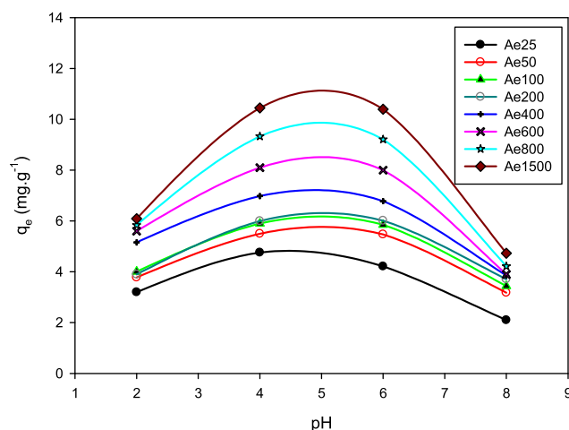
Fig. 4. Effect of pH on the capacity of Ni(II) adsorption of carbon aerogels throughout the range of R/C ratios. Co = 100 \text{ mg.L}^{-1} , T = 25^\circ \text{C} . 0.1 \text{ g}/50 \text{ mL} . Contact time = 120 minutes.
