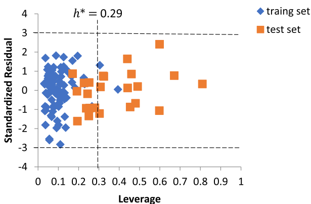
Fig. 3. Williams Plot, A plot of standardized residual versus Leverage of model 1.
