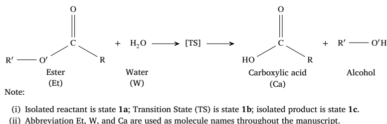
Scheme 1. The one-step reaction model in this study.
