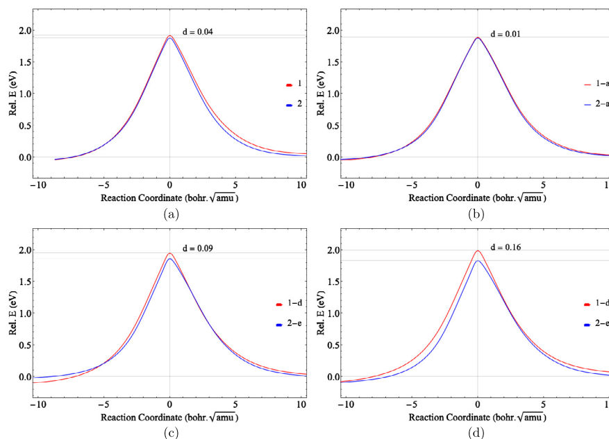
Fig. 6. Reaction path calculations based on the optimized geometry of [Et-W] complexes for the case of (a) Et1, (b) Et2, (c) Et3, and (d) Et4 with the conformations are shown in the legend. The peak of path is the saddle point which is the transition state (1b), to the left is the initial state (1a) and to the right is the final state (1c). The energy reference is the 1a of each system, so the height corresponds to the energy barrier of each reaction with d as the difference in energy barrier between two different conformers. (Table 11 lists the complete value of energy barrier for all reactions of interest.)
