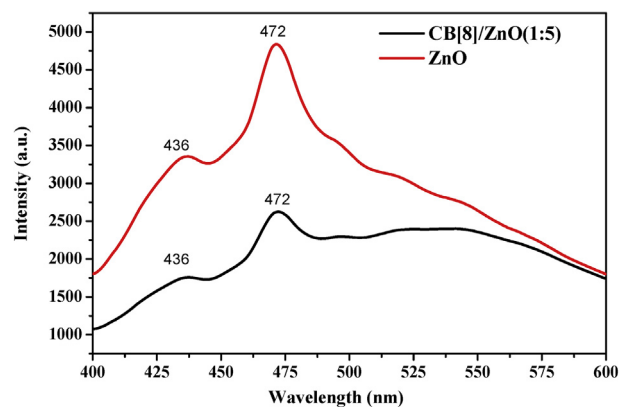
Fig. 8. Photoluminescence spectra of ZnO and CB[8]/ZnO composite.
