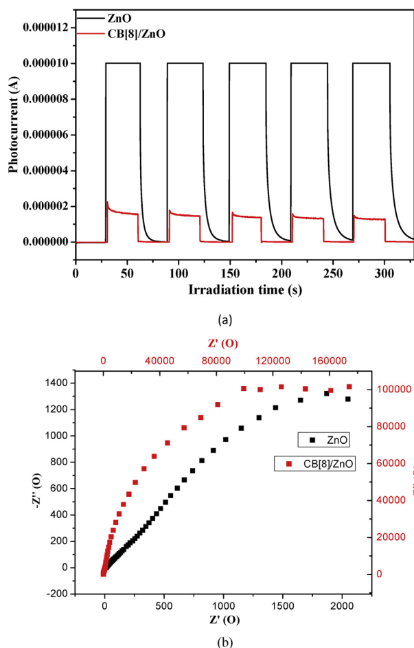
Fig. 9. The transient photocurrent responses (a) and Electrochemical impedance spectrum (b) of ZnO and CB[8]/ZnO composite.
