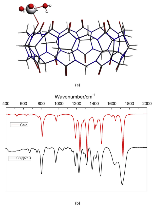
Fig. 4. The optimized ground state geometry of 1:1 CB[8]/ZnO on the B3LYP/LanL2dz/6-31G(d) level of theory (a), and a comparison of the experimental and simulated IR spectra (b).
