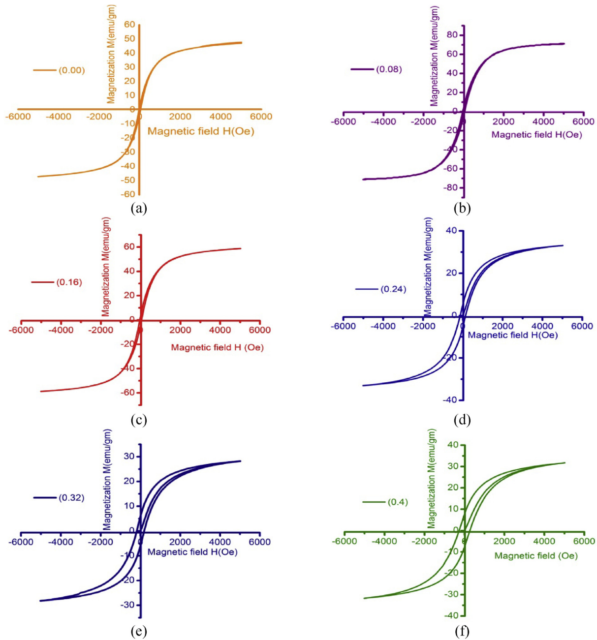
Fig. 10. (a)–(f). Hysteresis curves of M-H Zr and Co substituted \text{Ni}_{0.5}\text{Zn}_{0.5}\text{Zr}_x\text{Co}_{1-x}\text{Fe}_{2-2x}\text{O}_4 ( x = 0.00, 0.08, 0.16, 0.24, 0.32 and 0.4 ).
