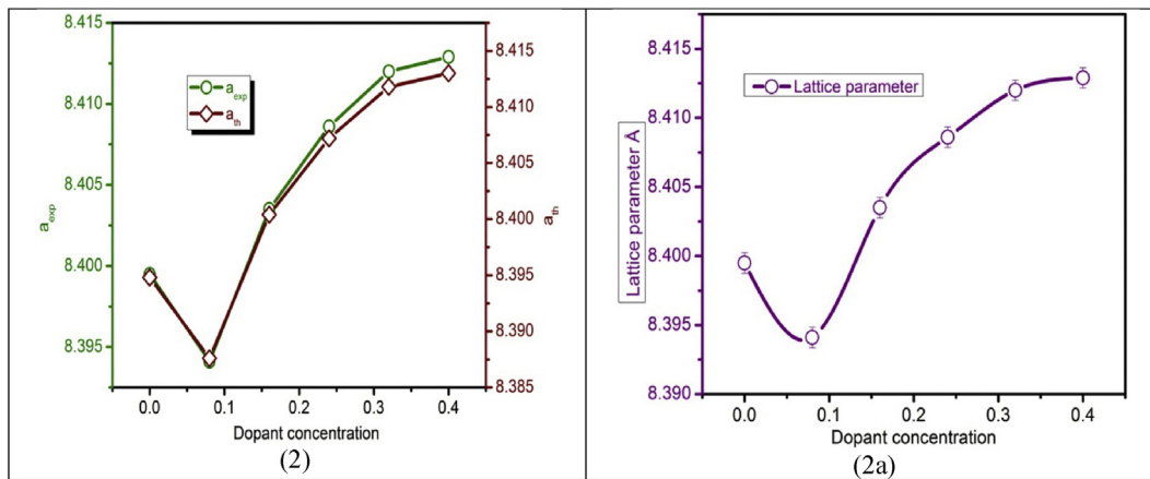
Fig. 2. Variation of experimental and theoretical lattice parameter with dopant concentration and Fig. 2(a) error bars of lattice parameter variation with dopant concentration.
