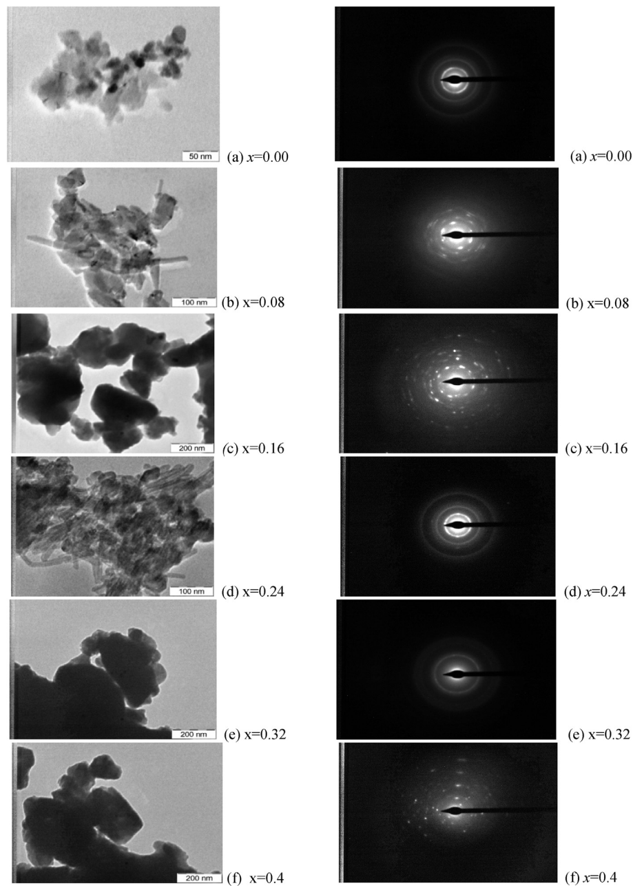
Fig. 6. (a)–(f). Transmission electron micrographs of \text{Ni}_{0.5}\text{Zn}_{0.5}\text{Zr}_x\text{Co}_x\text{Fe}_{2-2x}\text{O}_4 along with selected area Electron diffraction patterned of the samples ( x = 0.00, 0.08, 0.16, 0.24, 0.32 and 0.4 ).
