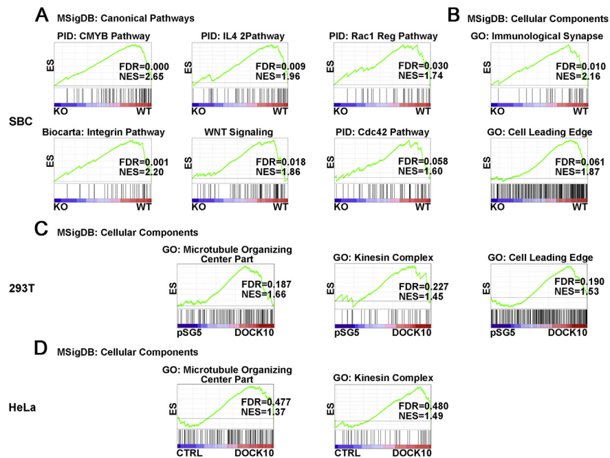
Fig. 2. Canonical pathways and cellular components of the MSigDB regulated by DOCK10 in SBC, 293T and HeLa cells, according to GSEA. (A) Canonical pathways in SBC. (B) Cellular components in SBC. (C) Cellular components in 293T cells. (D) Cellular components in HeLa cells. In SBC, KO was the reference condition for WT . In 293T and HeLa, pSG5 and CTRL were the reference conditions for DOCK10 , respectively. ES, enrichment score; FDR, false discovery rate; GO, gene ontology; NES, normalized enrichment score; PID, Protein Interaction database.
