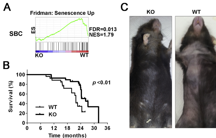
Fig. 3. Survival analysis of Dock10-KO mice and WT mice. (A) Enrichment of the Fridman: Senescence Up gene set in WT condition compared to the reference KO condition according to GSEA. ES, enrichment score; FDR, false discovery rate; NES, normalized enrichment score. (B) Survival analysis of two cohorts of Dock10-KO mice (N = 26) and WT mice (N = 28) using GraphPad Prism software. (C) Coat of 24-month-old Dock10-KO mice and WT mice, showing reduced hair loss in KO mice.
