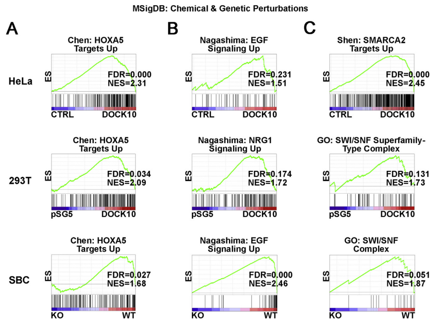
Fig. 1. Common and related signatures of the Chemical & Genetic Perturbations collection of the MSigDB associated to expression of DOCK10 in HeLa cells, 293T cells and SBC, according to GSEA. (A) Chen: HOXA5 Targets Up gene set. (B) Nagashima: EGF Signaling Up or closely related Nagashima: NRG1 Signaling Up gene sets. (C) Shen: SMARCA2 Targets Up gene set or the related GO: SWI/SNF Superfamily-Type Complex or GO: SWI/SNF Complex gene sets. In HeLa and 293T, CTRL and pSG5 were the reference conditions for DOCK10 , respectively. In SBC, KO was the reference condition for WT. ES, enrichment score; FDR, false discovery rate; GO, gene ontology; NES, normalized enrichment score.
