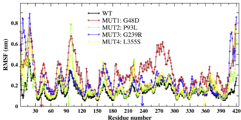
Fig. 3. RMSF plot of native and all mutants (G49D, P93L, G239R, and L355S) of PIGA protein.
