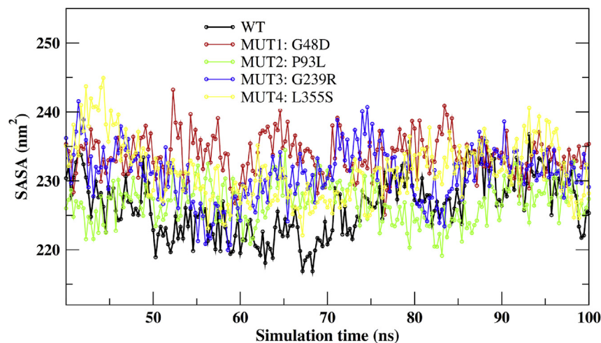
Fig. 5. SASA plot of native and all mutants (G49D, P93L, G239R, and L355S) of PIGA protein.
