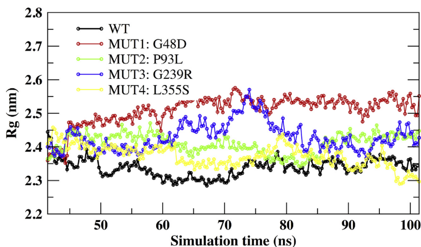
Fig. 4. Rg plot of native and investigated mutants (G49D, P93L, G239R, and L355S) of PIGA protein.
