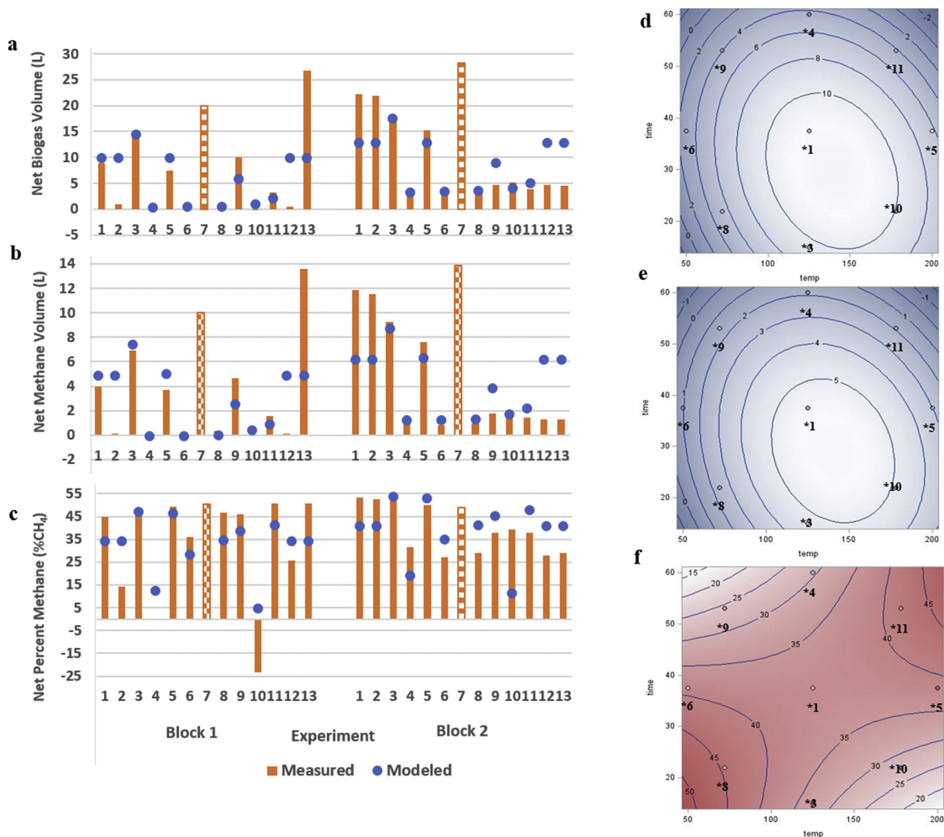
Fig. 1. a-c: Measured and modeled values for the net biogas volume, net methane volume, and the net percent methane based on response surface methodology. Treatment 7 is the positive control and was not included in the central composite rotatable design. Both blocks were analyzed together. For Fig. 1c, Block 1, Experiment 10 produced less gas than the inoculum, its net percent methane is negative. See Tables 2 and 3 for the temperature and duration combination for each treatment. Fig. 1d-f: Contour plots showing the biogas volume, which peaked at about 150 °C, 50 min; the methane volume, which peaked at about 150 °C, 40 min; and the change in percent methane, all in response to pretreatment temperature and duration. The numbers with asterisks are the numbers of the experiments.
