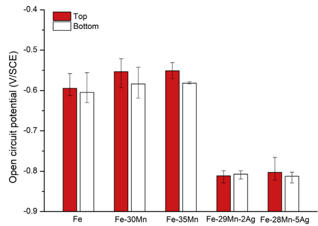
Fig. 12. OCP value of pressed and sintered Fe, Fe-30Mn, Fe-35Mn, Fe-29Mn-2Ag and Fe-28Mn-5Ag measured over 1 h. Error bars are representative of the maximum and minimum value obtained for n = 3 samples.
