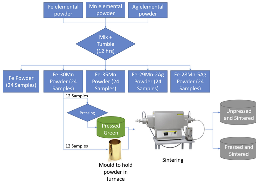
Fig. 1. Schematic diagram of the sample preparation procedure.
