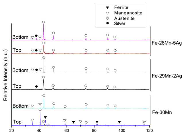
Fig. 4. X-Ray diffractograms of the top and bottom surfaces of polished, pressed and sintered Fe-30Mn, Fe-29Mn-2Ag and Fe-28Mn-5Ag coupons.
