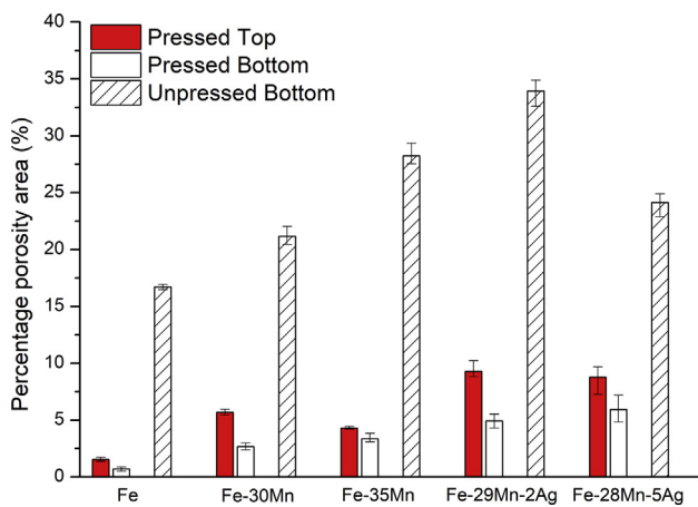
Fig. 11. Percentage porosity area for the pressed and non-pressed samples ( n = 3 ). Error bars represent the maximum and minimum porosity values.
