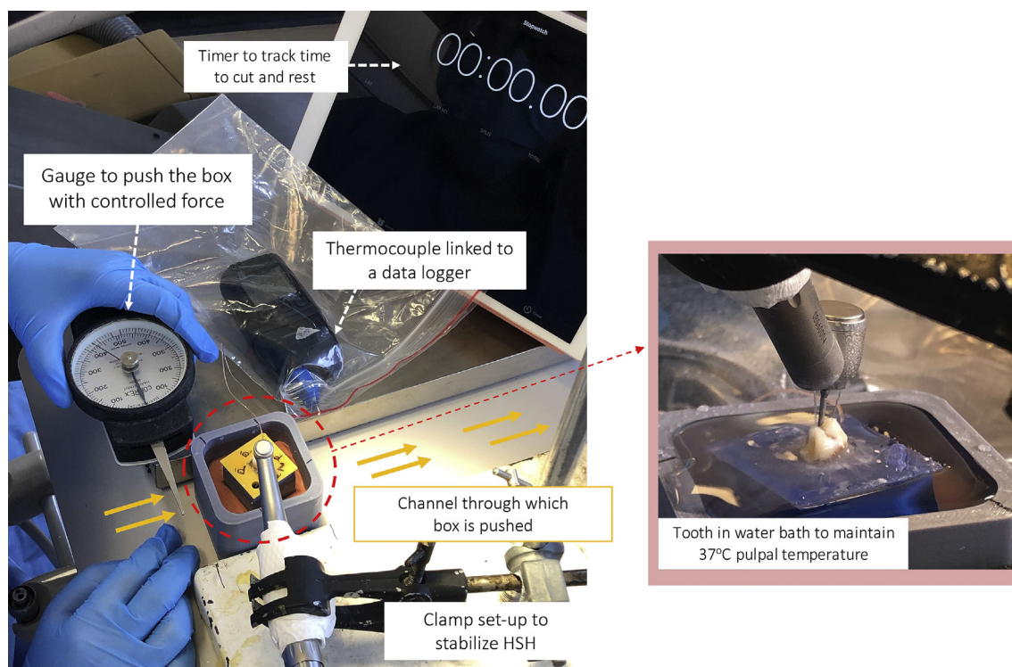
Fig. 2. Testing apparatus and experimental set-up.
