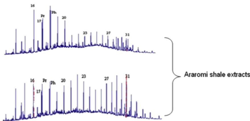
Fig. 9. Gas chromatograms of representative saturated hydrocarbon fractions of the Araromi shale (samples GB314 and GB 307) extracts showing how n-alkane and isoprenoid distributions in the Araromi shale. m/z 217 mass chromatograms.
