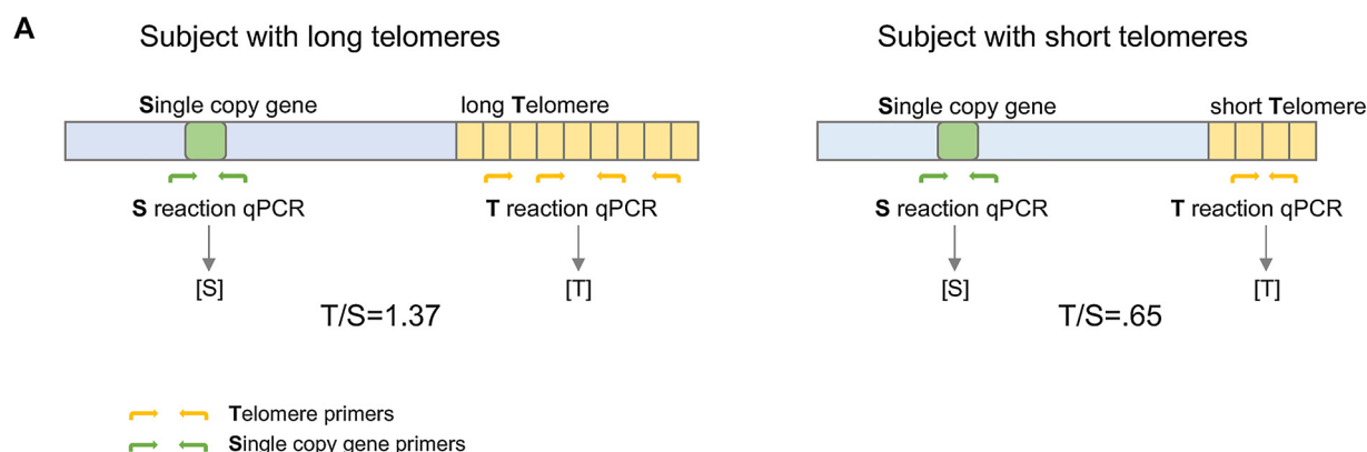
Fig. 1. A. Schematic diagram of qPCR telomere length measurement as described in Cawthon 2002 (Cawthon, 2002). Examples of two subjects, with high and low T/S ratios, representing long and short average telomere length, are presented. These numbers are arbitrary, but are in the typical range of values for normal, healthy adults when a pooled human genomic DNA is used as the reference standard. B. Schematic diagram of monochrome multiplex quantitative PCR method (mmQPCR) for telomere length measurement, adapted from the original publication (Cawthon, 2009).
