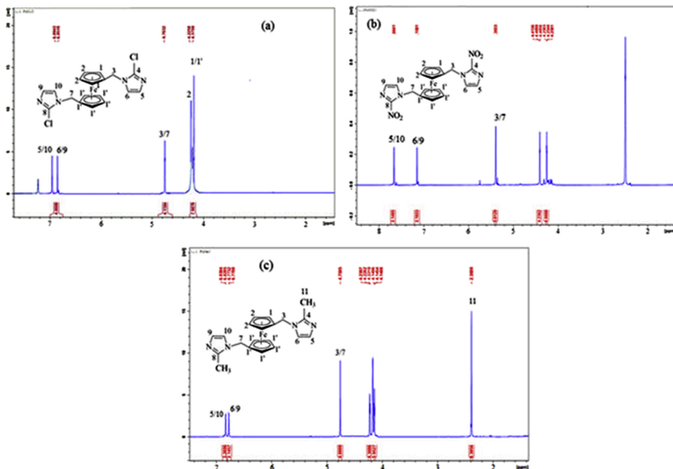
Fig. 1. ^1\text{H} -NMR of compounds (a) 4 (b) 5 and (c) 6.
