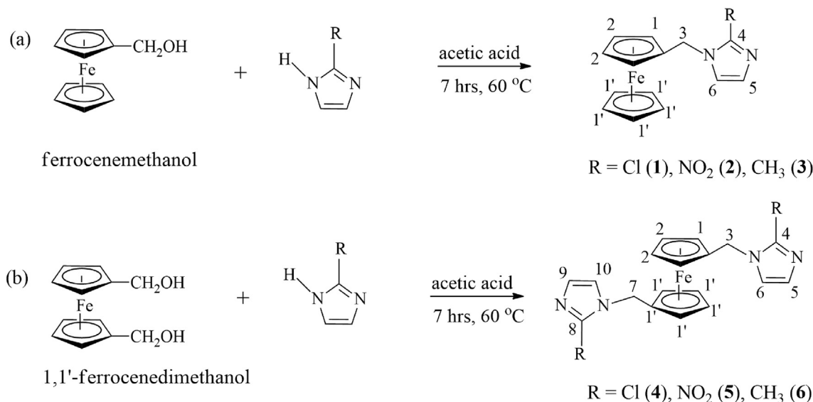
Scheme 1. Reaction schemes of (a) ferrocenemethanol and (b) 1,1'-diferoenemethanol for the synthesis of compounds 1–6.
