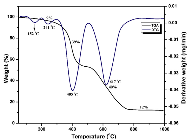
Fig. 3. TGA and DTG curves of mlc3 complex.
