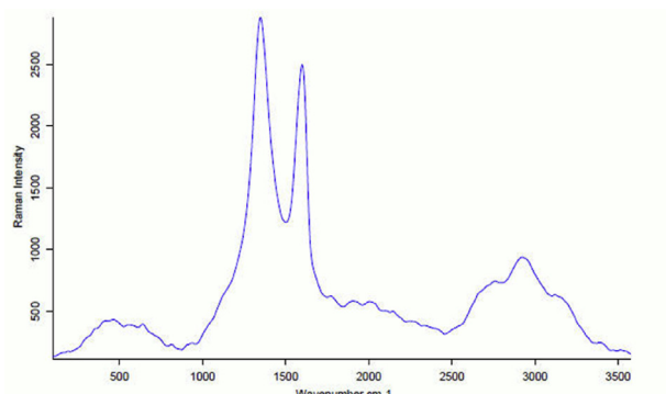
Fig. 2. Raman spectrum of Graphene oxide.
