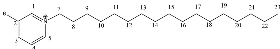
Scheme 1. Numbering of carbon and proton atoms of surfactants (I & II) for interpretation of ^1\text{H} - and ^{13}\text{C} -NMR.
