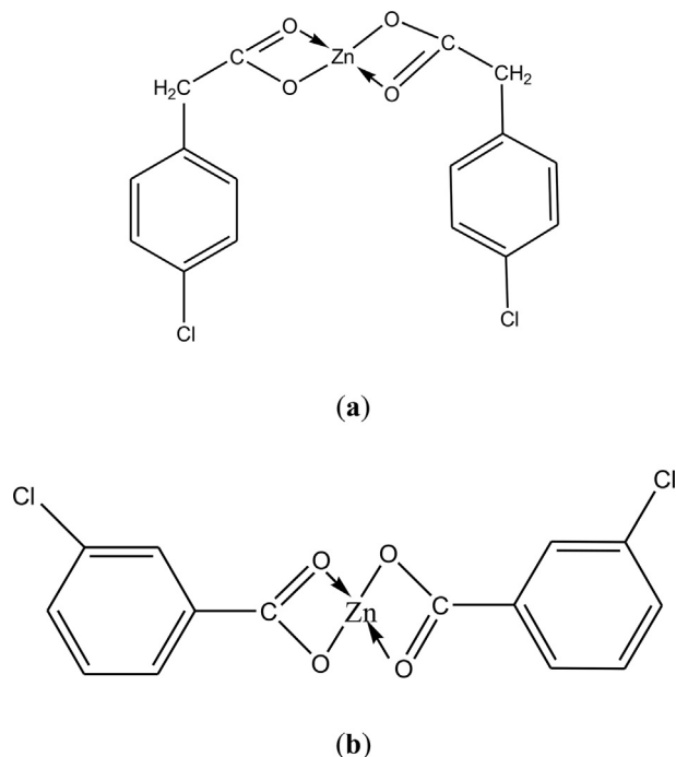
Fig. 7. Zn (II) Complexes a) [Zn (L 1 ) 2 ] b) [Zn (L 2 ) 2 ].
