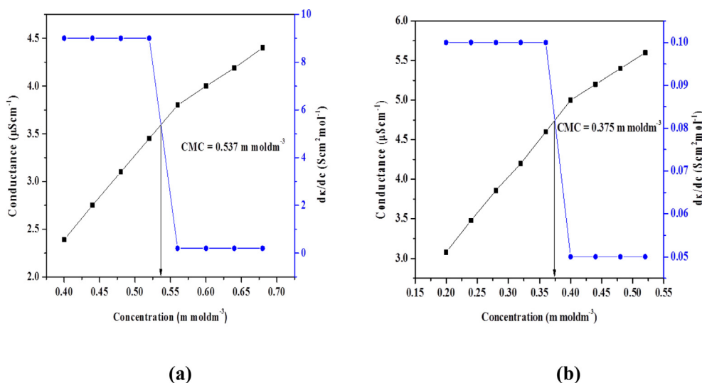
Fig. 8. [Zn (L 1 ) 2 ] interactions with a) compound I and b) compound II.
