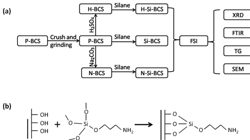
Figure 2. The schematic diagram of grafting APS on BCS (a), and proposed mechanism of BCS reacting with APS (b).
