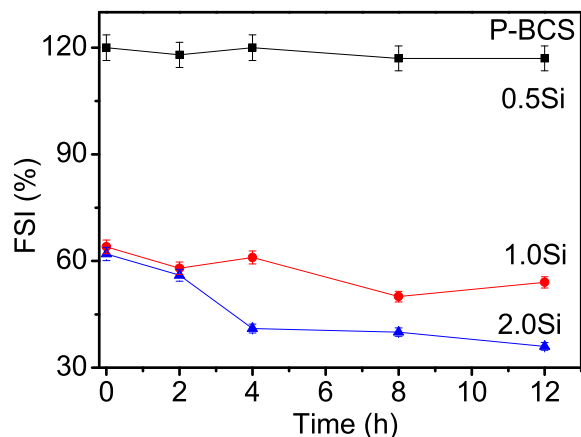
Figure 3. The FSI plots of pristine BCS, and its surface-modified samples by APS with different dosages (0.5Si, 1.0Si and 2.0Si means the use of APS are 0.5, 1.0 and 2.0 times of CEC (84.3 meq/100 g)).
