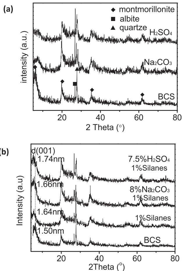
Figure 7. (a) The XRD profiles of BCS treated with \text{H}_2\text{SO}_4 and \text{Na}_2\text{CO}_3 solutions; (b) The XRD patterns of H-BCS or N-BCS modified with APS.
