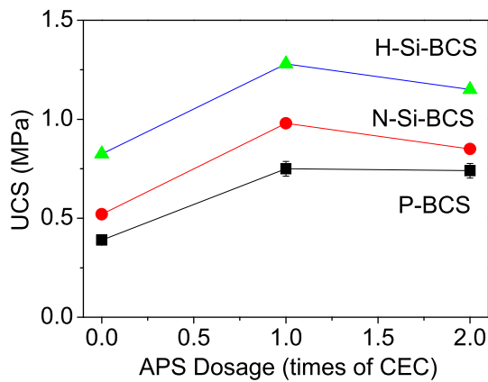
Figure 6. APS dosage effects on the UCS of P-BCS and those treated with \text{H}_2\text{SO}_4 (H-Si-BCS) or \text{Na}_2\text{CO}_3 (N-Si-BCS).
