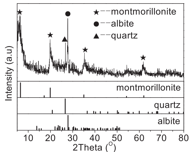
Figure 1. XRD pattern of the pristine BCS and indexed phases of major minerals (montmorillonite, quartz and albite).
