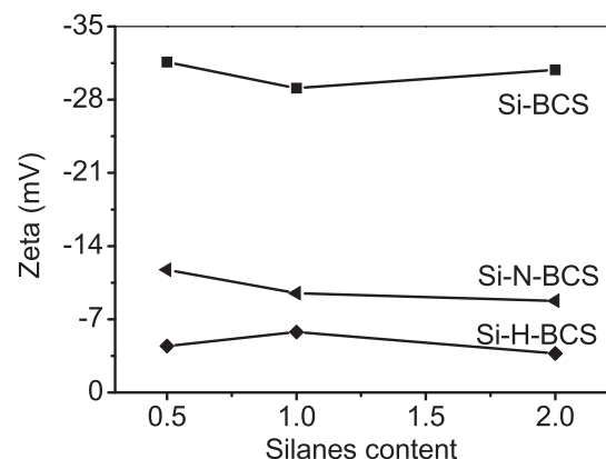
Figure 11. The Zeta potential of the BCS and those treated samples.
