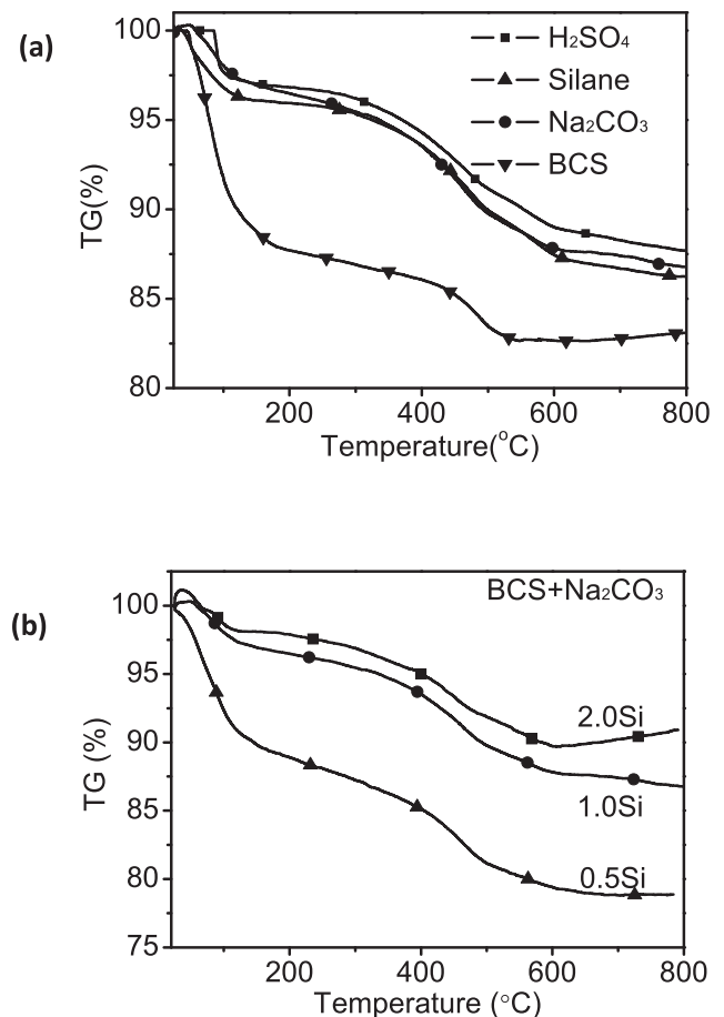
Figure 9. (a) TG curves of pristine BCS and modified BCS with different means (b) TG curves of different content of modified BCS pre-treated with \text{Na}_2\text{CO}_3 .
