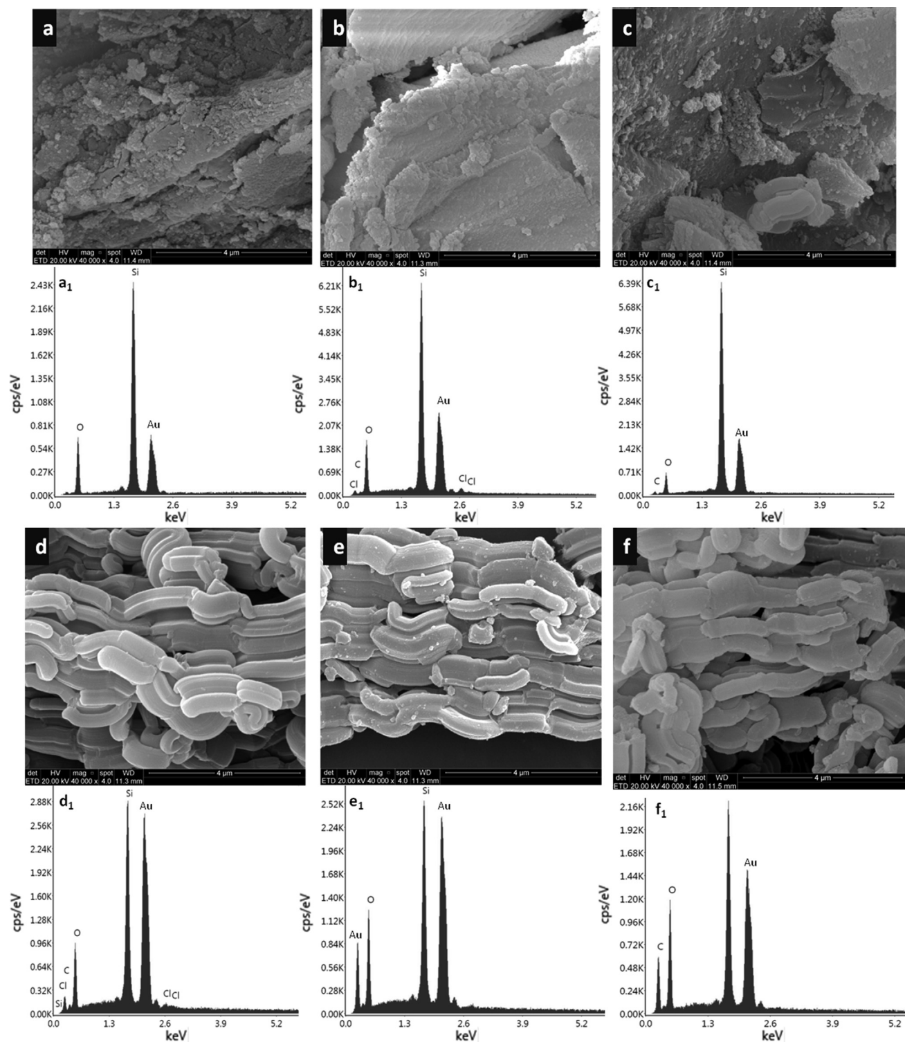
Fig. 4. Field emission scanning electron micrographs: (a) SIL (b) SIL-Cl (c) SIL-OAc (d) SBA (e) SBA-Cl (f) SBA-OAc and EDS: (a 1 ) SIL (b 1 ) SIL-Cl (c 1 ) SIL-OAc (d 1 ) SBA (e 1 ) SBA-Cl (f 1 ) SBA-OAc.
