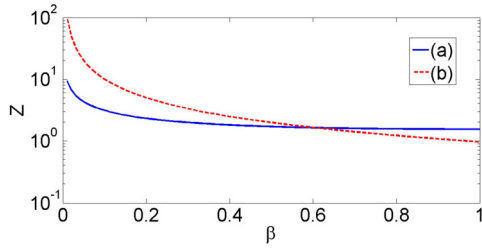
Fig. 5. Comparison of the partition function between (a) Z and (b) Z_0 for the parameter k = -0.90 .
