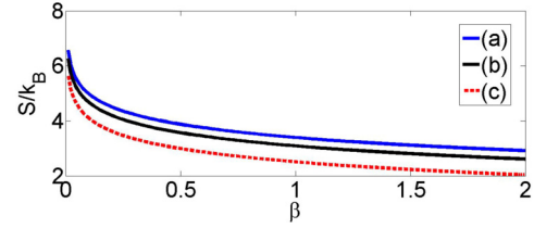
Fig. 8. Plot of the vibrational entropy S as function of \beta for (a) k = -0.25 , (b) k = -0.39 and (c) k = -0.90 .
