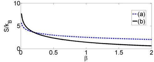
Fig. 9. Comparison of the vibrational entropy between (a) the variable mass system for k = -0.90 and (b) the linear oscillator.
