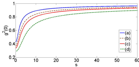
Fig. 3. Plot of the second order correlation function as a function of the coherent state parameter s for (a) k = -0.10 , (b) k = -0.25 , (c) k = -0.39 and (d) k = -0.90 .
