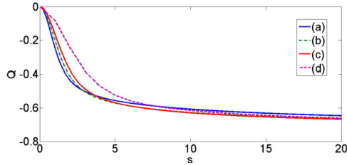
Fig. 2. Plot of the Mandel parameter as function of the coherent states parameter s for (a) k = -0.10 , (b) k = -0.25 , (c) k = -0.39 and (d) k = -0.90 .
