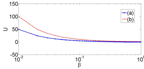
Fig. 7. Plot showing the comparison of the mean energy between (a) U and (b) U_0 for k = -0.90 .
