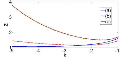
Fig. 4. Plot of the partition function Z as function of k for (a) \beta = 0.5 , (b) \beta = 1 and (c) \beta = 2 .
