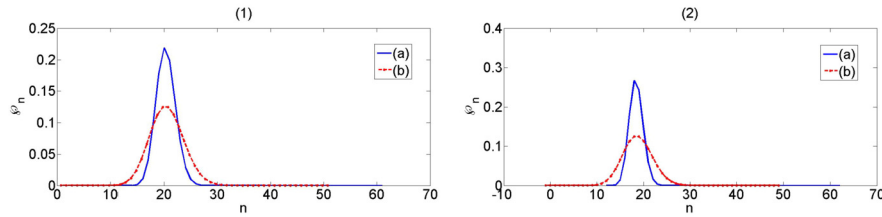
Fig. 1. Plot of the probability distribution for (a) the nonlinear oscillator and (b) the linear oscillator as a function of quantum number n with |s| = 20 for (1) k = -0.10 and (2) k = -0.90 .
