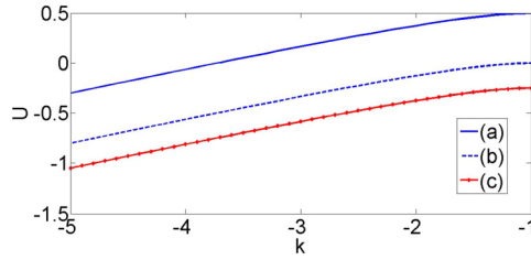
Fig. 6. Plot of the mean energy U as function of k for (a) \beta = 0.5 , (b) \beta = 1 and (c) \beta = 2 .
