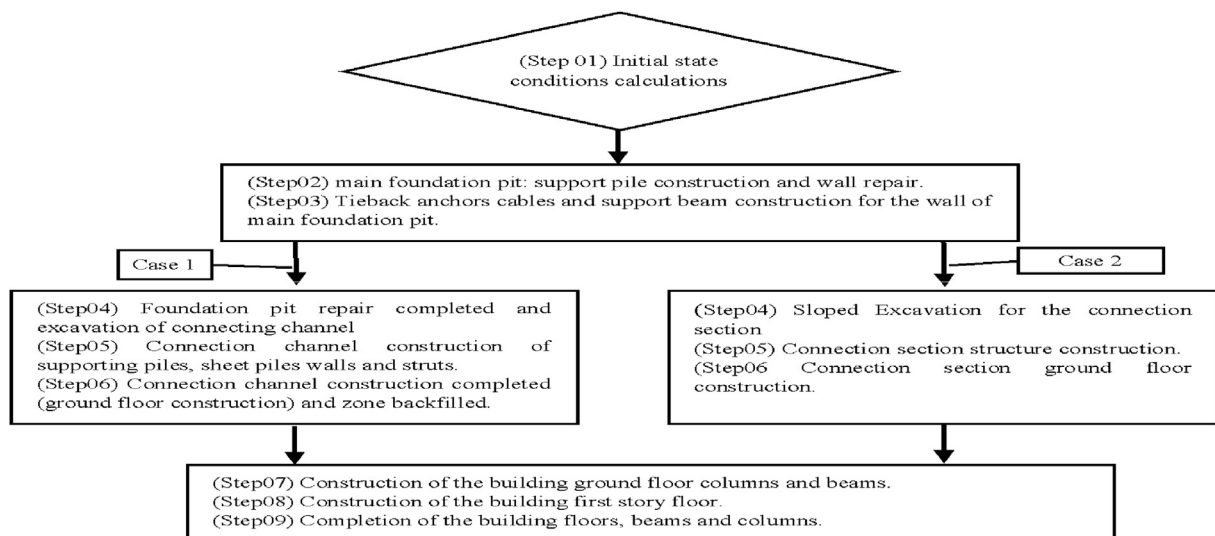
Fig. 6. Construction procedure.
