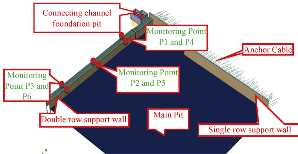
Fig. 3. Finite element model of foundation pit structure.
