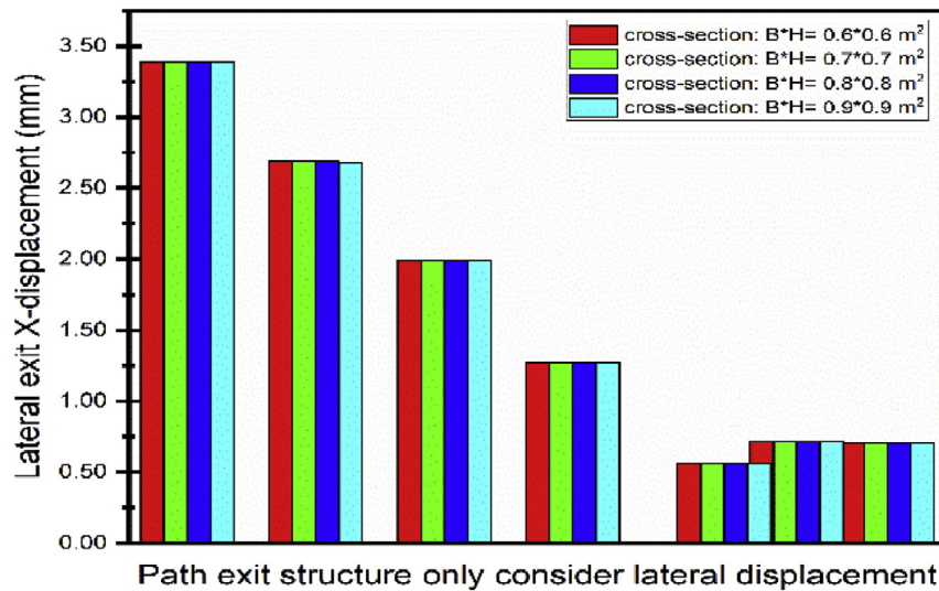
Fig. 25. Displacement variation in exit structure path chosen.
