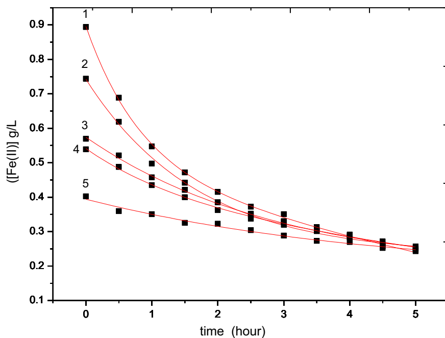
Fig. 7. Influence of time on ferrous concentrations at 25 °C. The dilution ratio: 1, 2.1; 2, 2.3; 3, 2.6; 4, 3.1; 5, 3.9.
