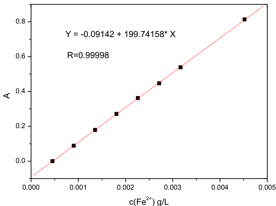
Fig. 3. The effect of c(\text{Fe}^{2+}) with 1,10-Phenanthroline on A.
