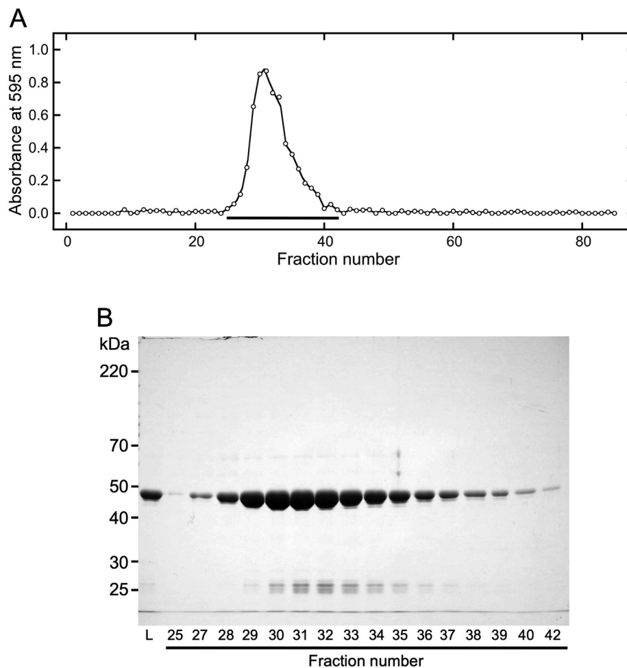
Figure 4. Gel filtration chromatography of proteins in the suspension with NaCl. Canavalin in the sword bean extract was precipitated via the addition of \text{MgCl}_2 at a final concentration of 15 mM. Precipitated canavalin was suspended in 200 mM NaCl, and the suspension was separated into the supernatant and precipitate by centrifugation. Supernatant proteins (2 mL) were loaded onto a gel filtration column that was equilibrated with 200 mM NaCl at a flow rate of 0.5 mL/min. Eluted samples were collected in volumes of 1.5 mL. (A) The eluted samples were reacted with Bradford dye reagent and then measured at 595 nm. Black bars indicate fractions analyzed by SDS-PAGE. (B) The loaded (L) and eluted samples were subjected to SDS-PAGE (10% polyacrylamide). Numbers represent fraction numbers in panel A.
