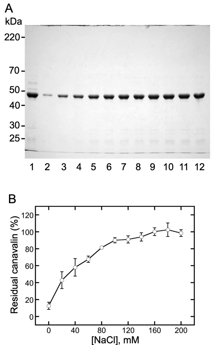
Figure 2. Effect of NaCl concentration on canavalin solubility. (A) Canavalin in the sword bean extract was precipitated via the addition of \text{MgCl}_2 at a final concentration of 15 mM and then suspended in 8 M urea (lane 1), distilled water (lane 2), or NaCl at concentrations of 20 mM (lane 3), 40 mM (lane 4), 60 mM (lane 5), 80 mM (lane 6), 100 mM (lane 7), 120 mM (lane 8), 140 mM (lane 9), 160 mM (lane 10), 180 mM (lane 11), and 200 mM (lane 12). Distilled water was used as the control (0 mM). Suspensions were separated into the supernatant and precipitate, and the supernatant was subjected to SDS-PAGE (10% polyacrylamide). (B) The proportion of residual canavalin in the supernatant was estimated from the band intensity using ImageJ. Data are expressed as the means \pm standard deviations of three independent replicates.
