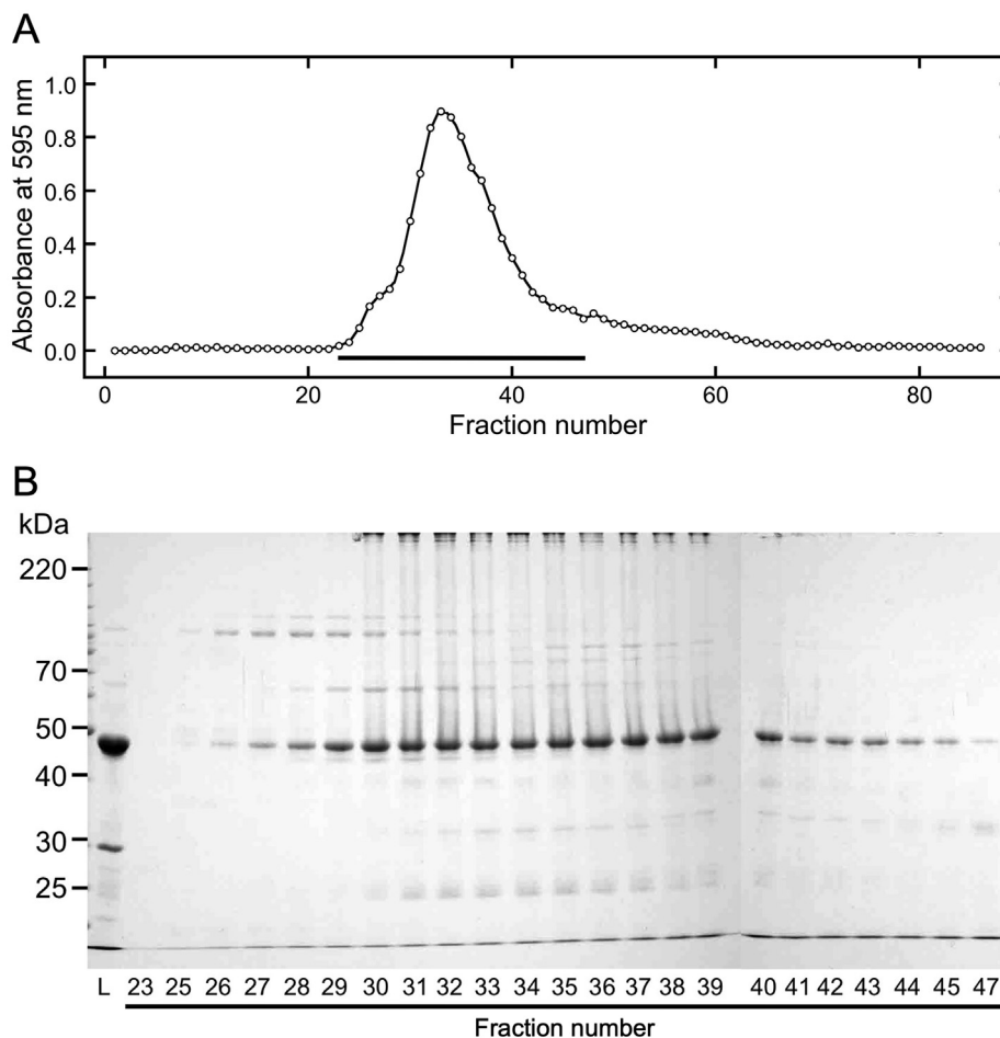
Figure 6. Gel filtration chromatography of proteins in the sword bean extract and \text{MgCl}_2 mixture. \text{MgCl}_2 was added to the sword bean extract at a final concentration of 60 mM. The \text{MgCl}_2 mixture was separated into the supernatant and precipitate by centrifugation. Supernatant proteins (2 mL) were loaded onto a gel filtration column that was equilibrated with 60 mM \text{MgCl}_2 at a flow rate of 0.5 mL/min. Eluted samples were collected in volumes of 1.5 mL. (A) The eluted samples were reacted with Bradford dye reagent, and then measured at 595 nm. Black bars indicate fractions analyzed by SDS-PAGE. (B) The loaded (L) and eluted samples were subjected to SDS-PAGE (10% polyacrylamide). Numbers represent fraction numbers in panel A. Eluted samples were distinguished between fraction numbers 23–39 and 40–47 on different gel plates.
