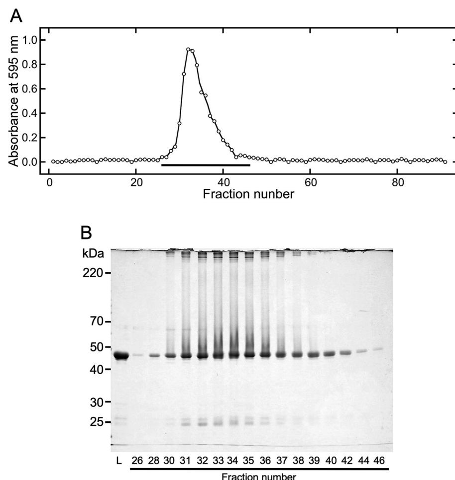
Figure 7. Gel filtration chromatography of proteins in the suspension with \text{MgCl}_2 . Canavalin in the sword bean extract was precipitated via the addition of \text{MgCl}_2 at a final concentration of 15 mM. Precipitated canavalin was suspended in 60 mM \text{MgCl}_2 , and the suspension was separated into the supernatant and precipitate by centrifugation. Supernatant proteins (2 mL) were loaded onto a gel filtration column that was equilibrated with 60 mM \text{MgCl}_2 at a flow rate of 0.5 mL/min. Eluted samples were collected in volumes of 1.5 mL. (A) The eluted samples were reacted with Bradford dye reagent and then measured at 595 nm. Black bars indicate fractions analyzed by SDS-PAGE. (B) The loaded (L) and eluted samples were subjected to SDS-PAGE (10% polyacrylamide). Numbers represent fraction numbers in panel A.
