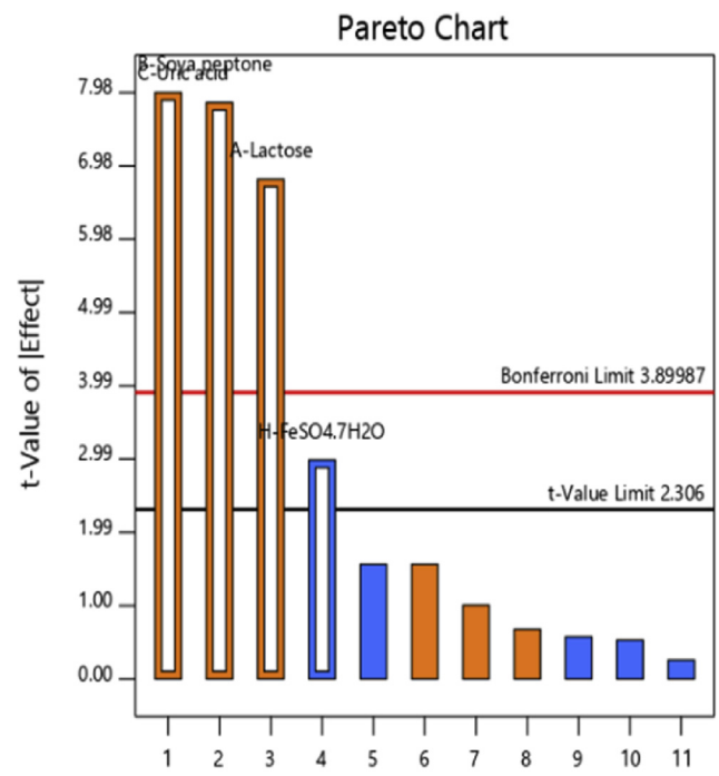
Fig. 5. Pareto chart showing four critical components affecting uricase yield.
