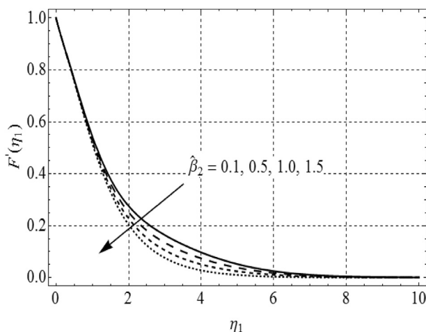
Fig. 2. F'(\eta_1) against \hat{\beta}_2 .
