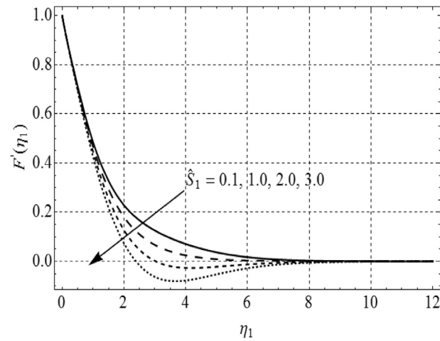
Fig. 3. F'(\eta_1) against \hat{S}_1 .
