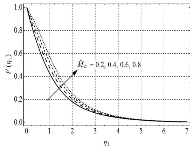
Fig. 4. F'(\eta_1) against \hat{M}_a .
