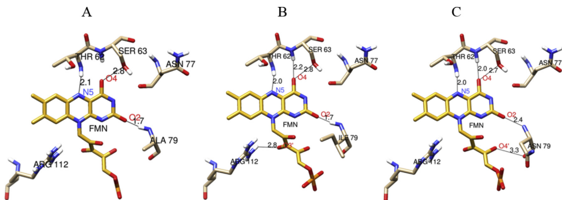
Fig. 6. Analysis of hydrogen bonds between FMN substrate and (A) wild-type DszD enzyme (B) A79I and (C) A79N using Chimera software.
