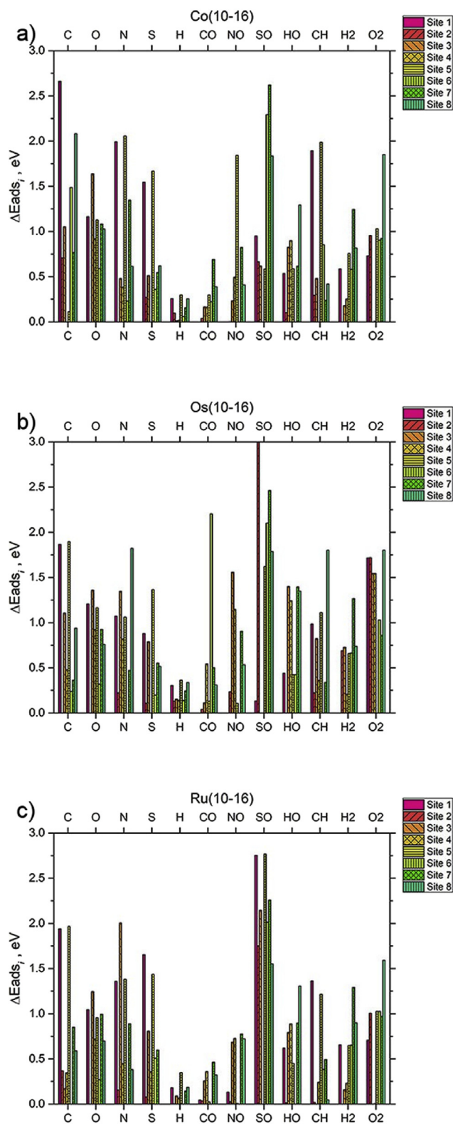
Fig. 6. Multiple Bar charts of relative adsorption energies, \Delta E_{ads_i} , in eV, for the species studied in this work on the stepped Co, Os, and Ru (10-16) surface(s). Data in this figure is identical to that in Figs. 3, 4, and 5, but shown aligned together to help guide the eye to similarities and differences. Data are grouped by adsorbate, on each surface. Figure SI3 and SI.4 show this same data, but grouped by site, and by surface/species, respectively. a) For the Co(10-16) surface, b) for the Os(10-16) surface c) for the Ru (10-16) surface.
