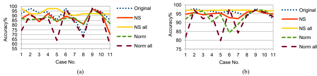
Fig. 23. Testing accuracy of FUGE F2F fusion on Testing 1 data (a) without and (b) with NSM and WS.
