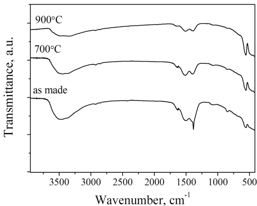
Fig. 6. FT-IR spectra (KBr disks) of the (\text{Ho}_{0.95}\text{La}_{0.05})_2\text{O}_3 nanopowder obtained from the SHS: “as made” and calcined in air at 700 and 900 °C for 3 h.
