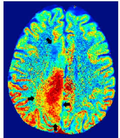
Fig. 2. Magnetic Resonance Spectrum at 7T (left). Axial GluCEST image (right) demonstrating increased GluCEST contrast in a glioma patient. From Neal et al. (2019).
