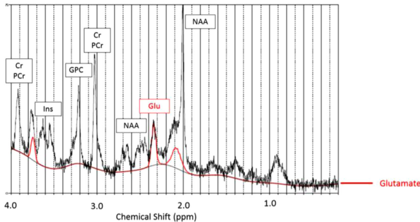
Fig. 2. Magnetic Resonance Spectrum at 7T (left). Axial GluCEST image (right) demonstrating increased GluCEST contrast in a glioma patient. From Neal et al. (2019).
