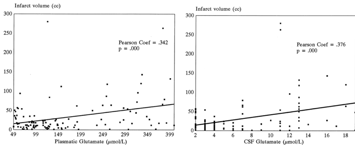
Fig. 1. The relationship between infarct volume and glutamate levels, from Castillo et al. (1996).
